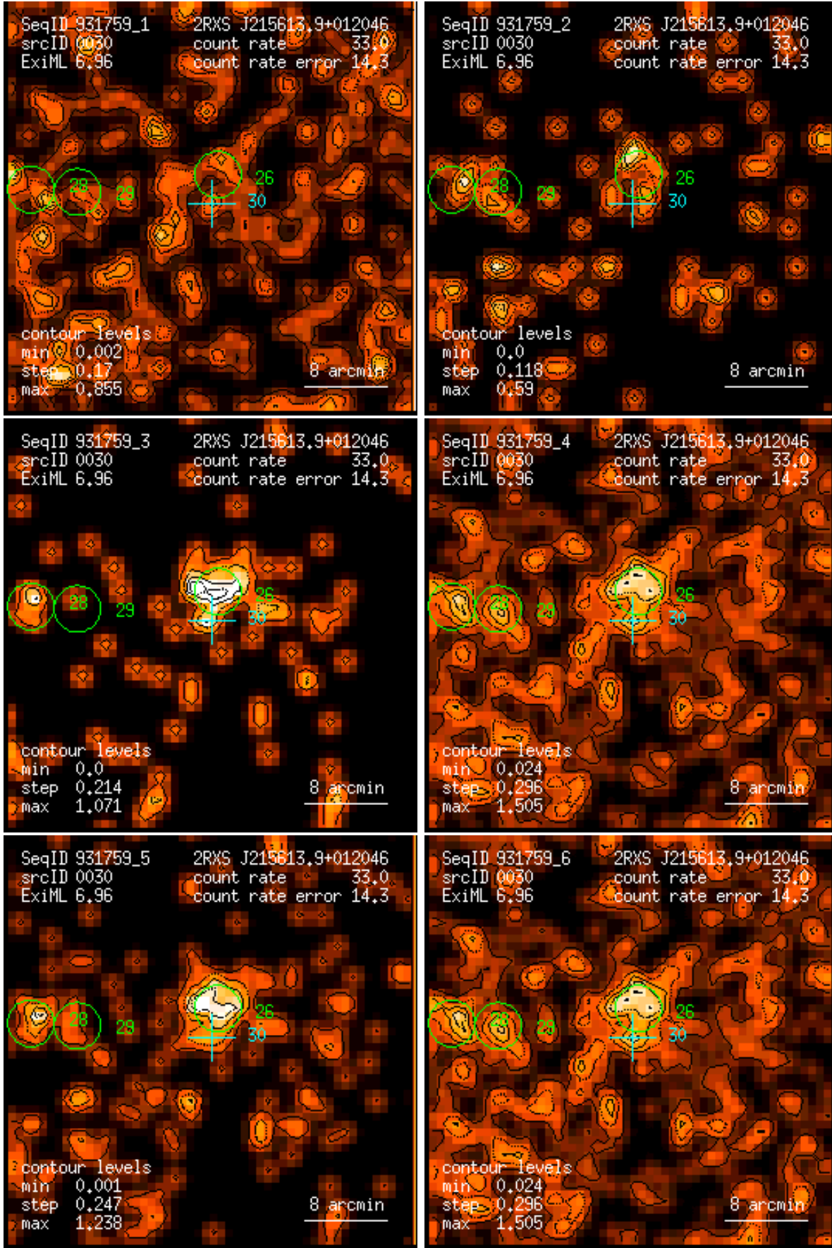
Figure 30: RASS 931759: detection 0030: band rate images, Gaussian filter: (1) PSPC channels 11 – 41, (2) 52 – 90, (3) 91 – 201, (4) 11 – 235, (5) 52 – 201, (6) 11 – 201. Broad band rates in counts/ks. Band rate contour levels in counts/ks/arcmin 2 .
