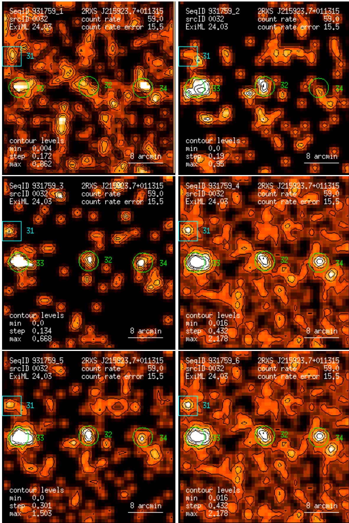
Figure 32: RASS 931759: detection 0032: band rate images, Gaussian filter: (1) PSPC channels 11 – 41, (2) 52 – 90, (3) 91 – 201, (4) 11 – 235, (5) 52 – 201, (6) 11 – 201. Broad band rates in counts/ks. Band rate contour levels in counts/ks/arcmin 2 .
