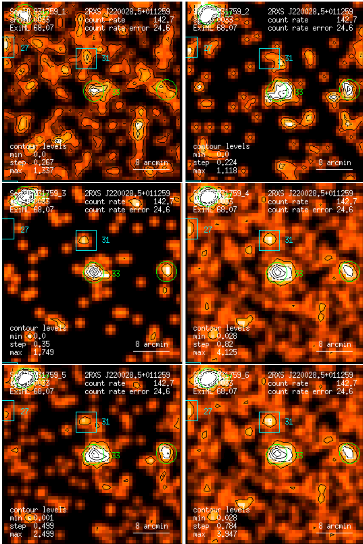
Figure 33: RASS 931759: detection 0033: band rate images, Gaussian filter: (1) PSPC channels 11 – 41, (2) 52 – 90, (3) 91 – 201, (4) 11 – 235, (5) 52 – 201, (6) 11 – 201. Broad band rates in counts/ks. Band rate contour levels in counts/ks/arcmin 2 .
