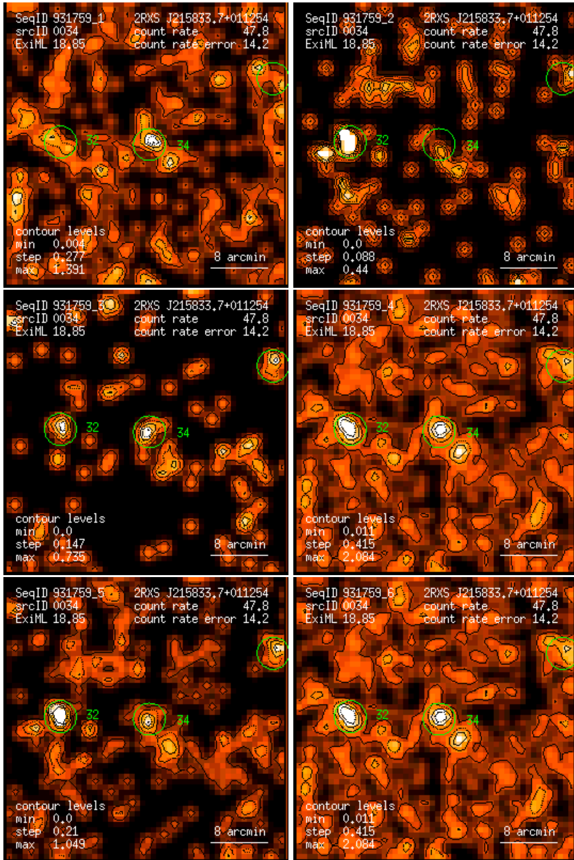
Figure 34: RASS 931759: detection 0034: band rate images, Gaussian filter: (1) PSPC channels 11 – 41, (2) 52 – 90, (3) 91 – 201, (4) 11 – 235, (5) 52 – 201, (6) 11 – 201. Broad band rates in counts/ks. Band rate contour levels in counts/ks/arcmin 2 .
