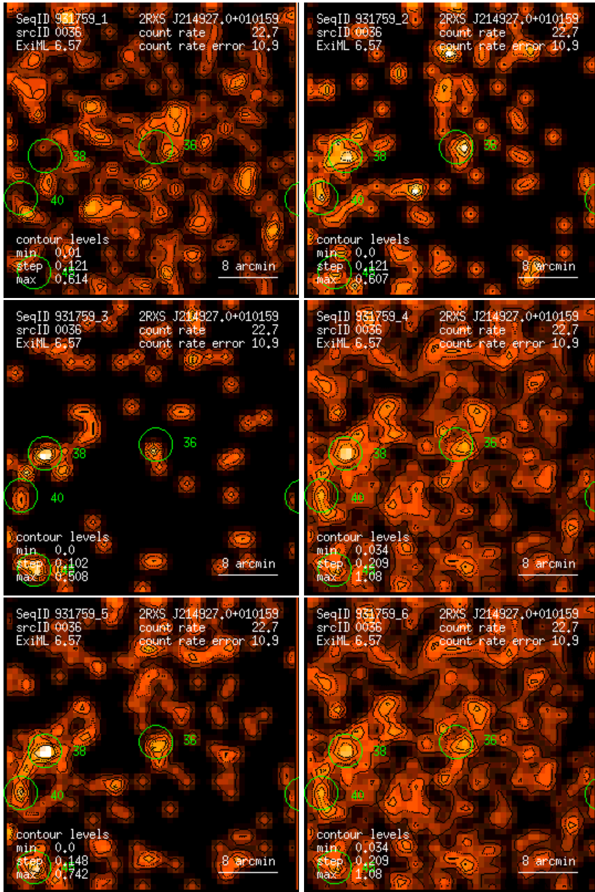
Figure 36: RASS 931759: detection 0036: band rate images, Gaussian filter: (1) PSPC channels 11 – 41, (2) 52 – 90, (3) 91 – 201, (4) 11 – 235, (5) 52 – 201, (6) 11 – 201. Broad band rates in counts/ks. Band rate contour levels in counts/ks/arcmin 2 .
