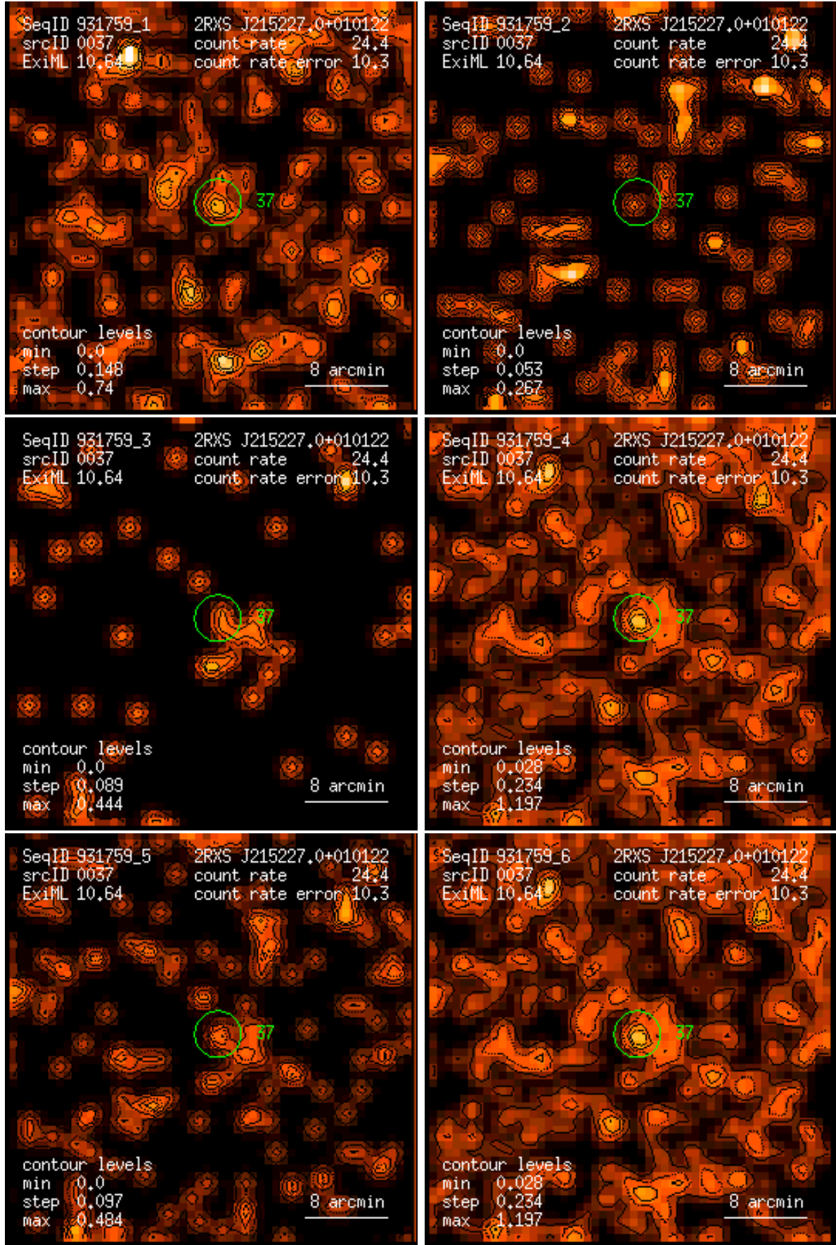
Figure 37: RASS 931759: detection 0037: band rate images, Gaussian filter: (1) PSPC channels 11 – 41, (2) 52 – 90, (3) 91 – 201, (4) 11 – 235, (5) 52 – 201, (6) 11 – 201. Broad band rates in counts/ks. Band rate contour levels in counts/ks/arcmin 2 .
