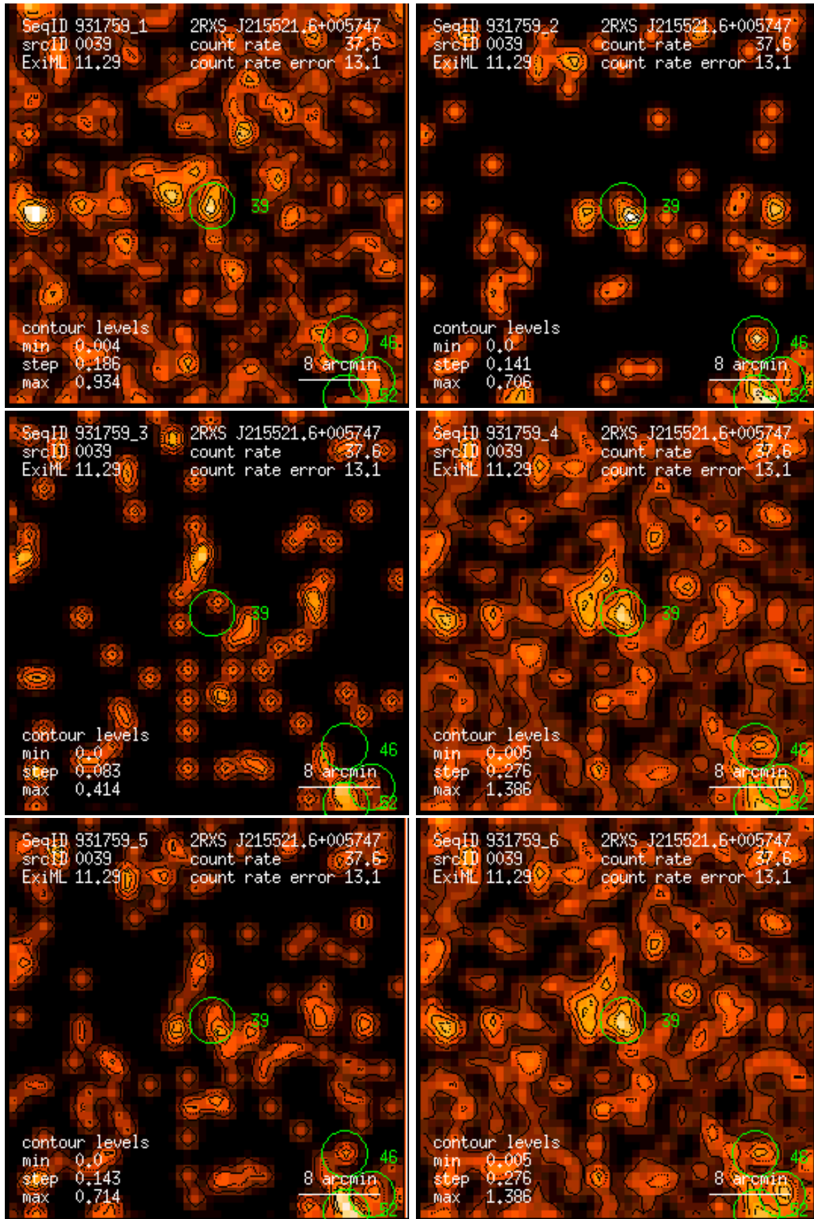
Figure 39: RASS 931759: detection 0039: band rate images, Gaussian filter: (1) PSPC channels 11 – 41, (2) 52 – 90, (3) 91 – 201, (4) 11 – 235, (5) 52 – 201, (6) 11 – 201. Broad band rates in counts/ks. Band rate contour levels in counts/ks/arcmin 2 .
