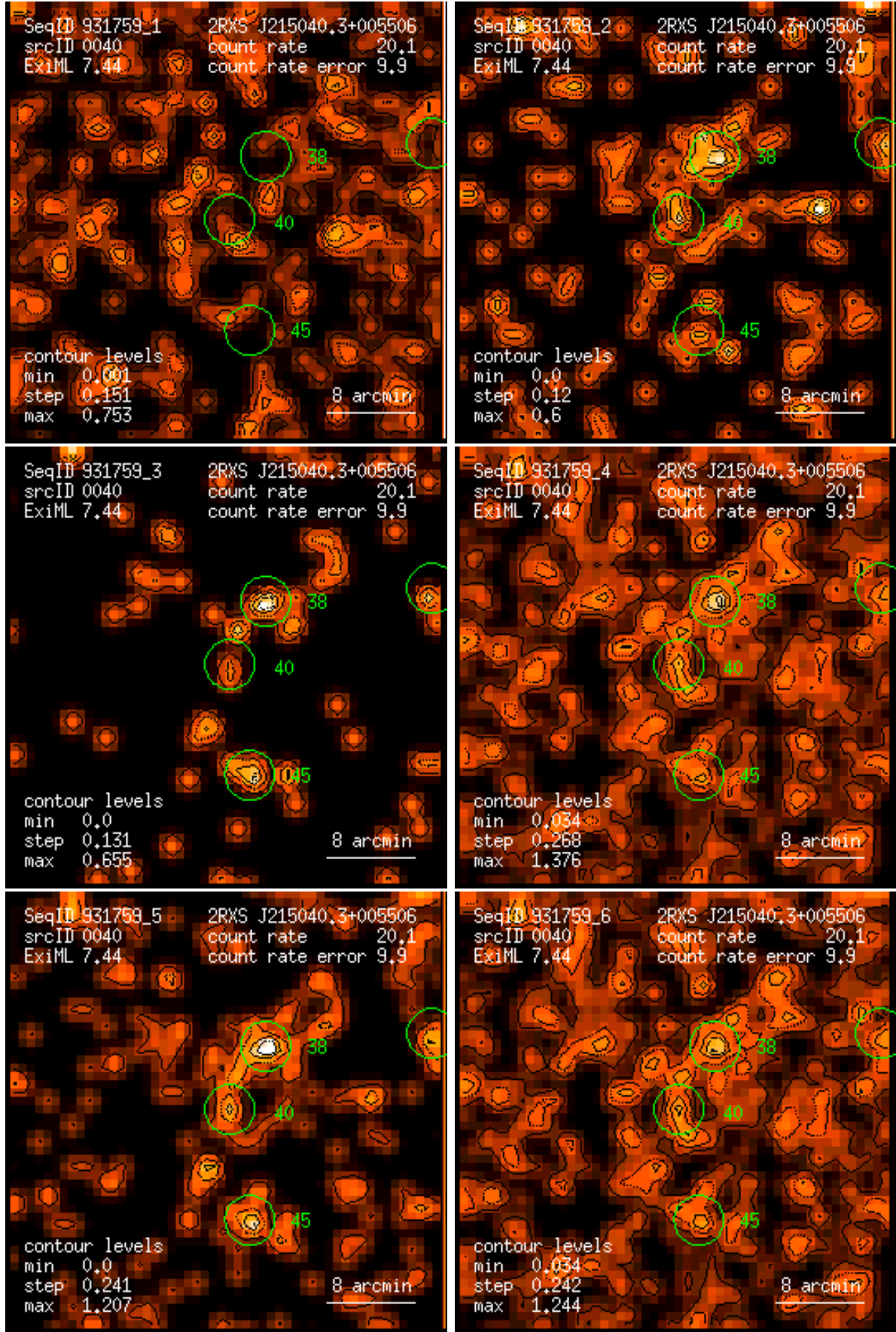
Figure 40: RASS 931759: detection 0040: band rate images, Gaussian filter: (1) PSPC channels 11 – 41, (2) 52 – 90, (3) 91 – 201, (4) 11 – 235, (5) 52 – 201, (6) 11 – 201. Broad band rates in counts/ks. Band rate contour levels in counts/ks/arcmin 2 .
