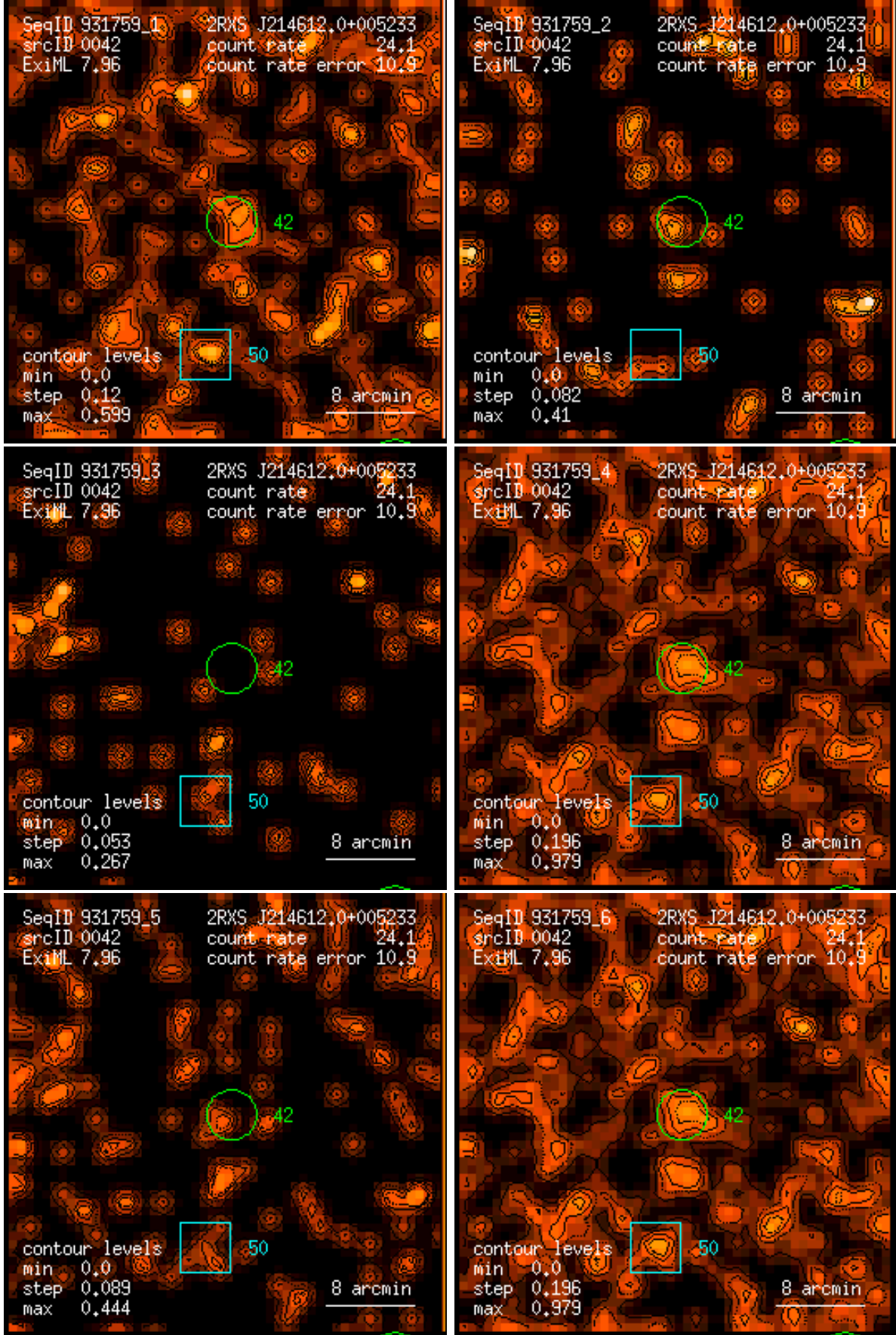
Figure 42: RASS 931759: detection 0042: band rate images, Gaussian filter: (1) PSPC channels 11 – 41, (2) 52 – 90, (3) 91 – 201, (4) 11 – 235, (5) 52 – 201, (6) 11 – 201. Broad band rates in counts/ks. Band rate contour levels in counts/ks/arcmin 2 .
