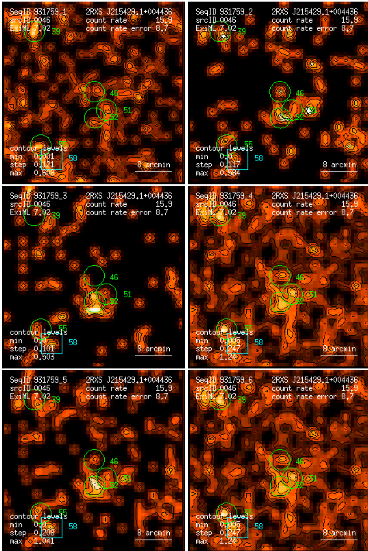
Figure 46: RASS 931759: detection 0046: band rate images, Gaussian filter: (1) PSPC channels 11 – 41, (2) 52 – 90, (3) 91 – 201, (4) 11 – 235, (5) 52 – 201, (6) 11 – 201. Broad band rates in counts/ks. Band rate contour levels in counts/ks/arcmin 2 .
