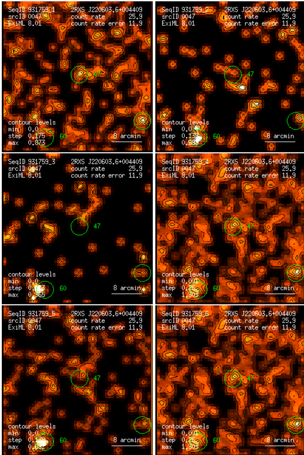
Figure 47: RASS 931759: detection 0047: band rate images, Gaussian filter: (1) PSPC channels 11 – 41, (2) 52 – 90, (3) 91 – 201, (4) 11 – 235, (5) 52 – 201, (6) 11 – 201. Broad band rates in counts/ks. Band rate contour levels in counts/ks/arcmin 2 .
