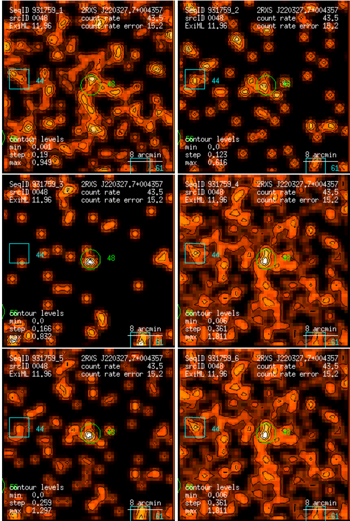
Figure 48: RASS 931759: detection 0048: band rate images, Gaussian filter: (1) PSPC channels 11 – 41, (2) 52 – 90, (3) 91 – 201, (4) 11 – 235, (5) 52 – 201, (6) 11 – 201. Broad band rates in counts/ks. Band rate contour levels in counts/ks/arcmin 2 .
