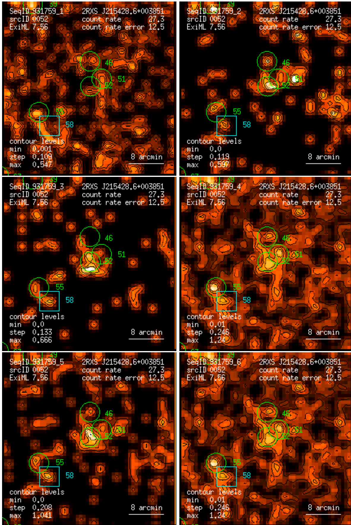
Figure 52: RASS 931759: detection 0052: band rate images, Gaussian filter: (1) PSPC channels 11 – 41, (2) 52 – 90, (3) 91 – 201, (4) 11 – 235, (5) 52 – 201, (6) 11 – 201. Broad band rates in counts/ks. Band rate contour levels in counts/ks/arcmin 2 .
