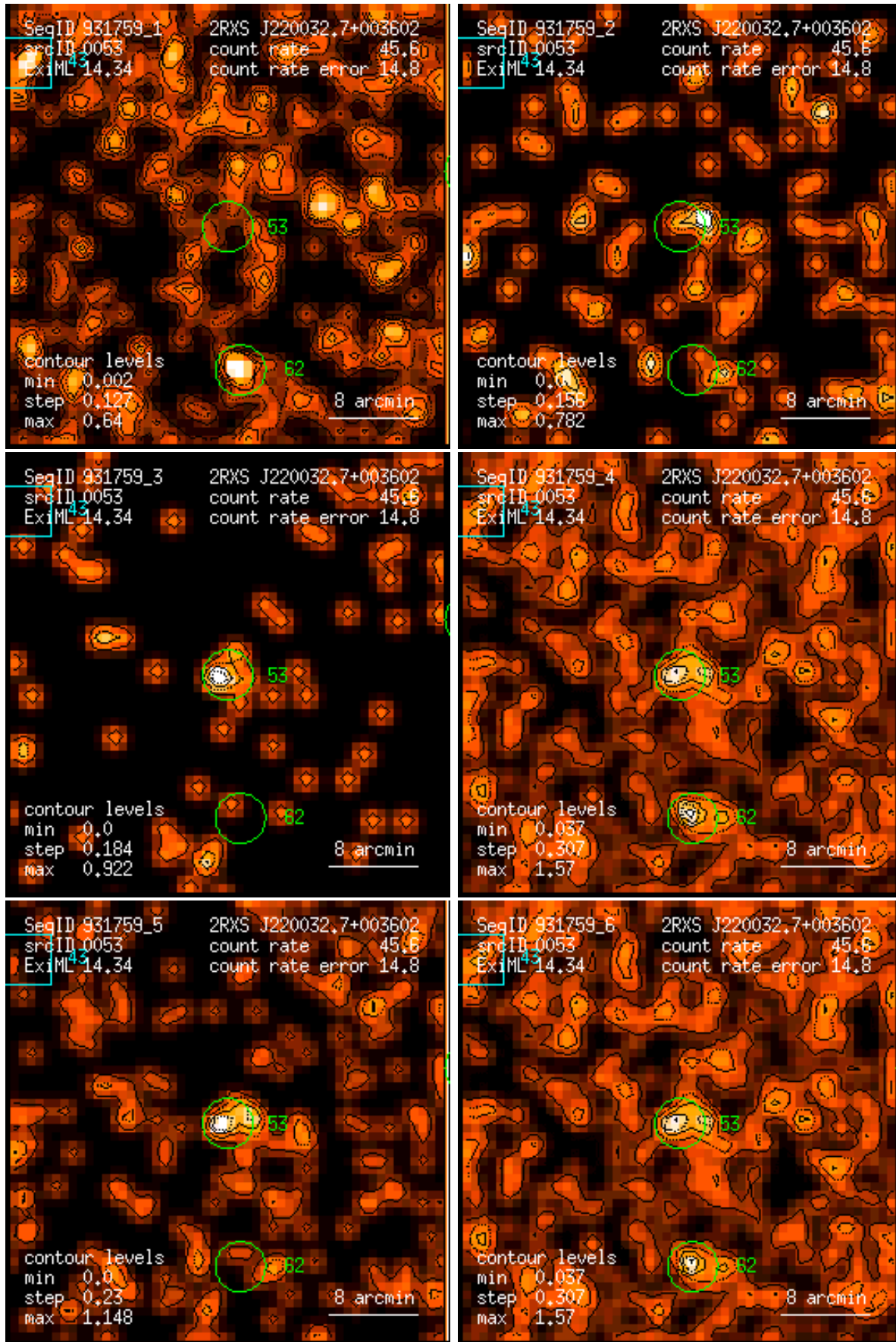
Figure 53: RASS 931759: detection 0053: band rate images, Gaussian filter: (1) PSPC channels 11 – 41, (2) 52 – 90, (3) 91 – 201, (4) 11 – 235, (5) 52 – 201, (6) 11 – 201. Broad band rates in counts/ks. Band rate contour levels in counts/ks/arcmin 2 .
