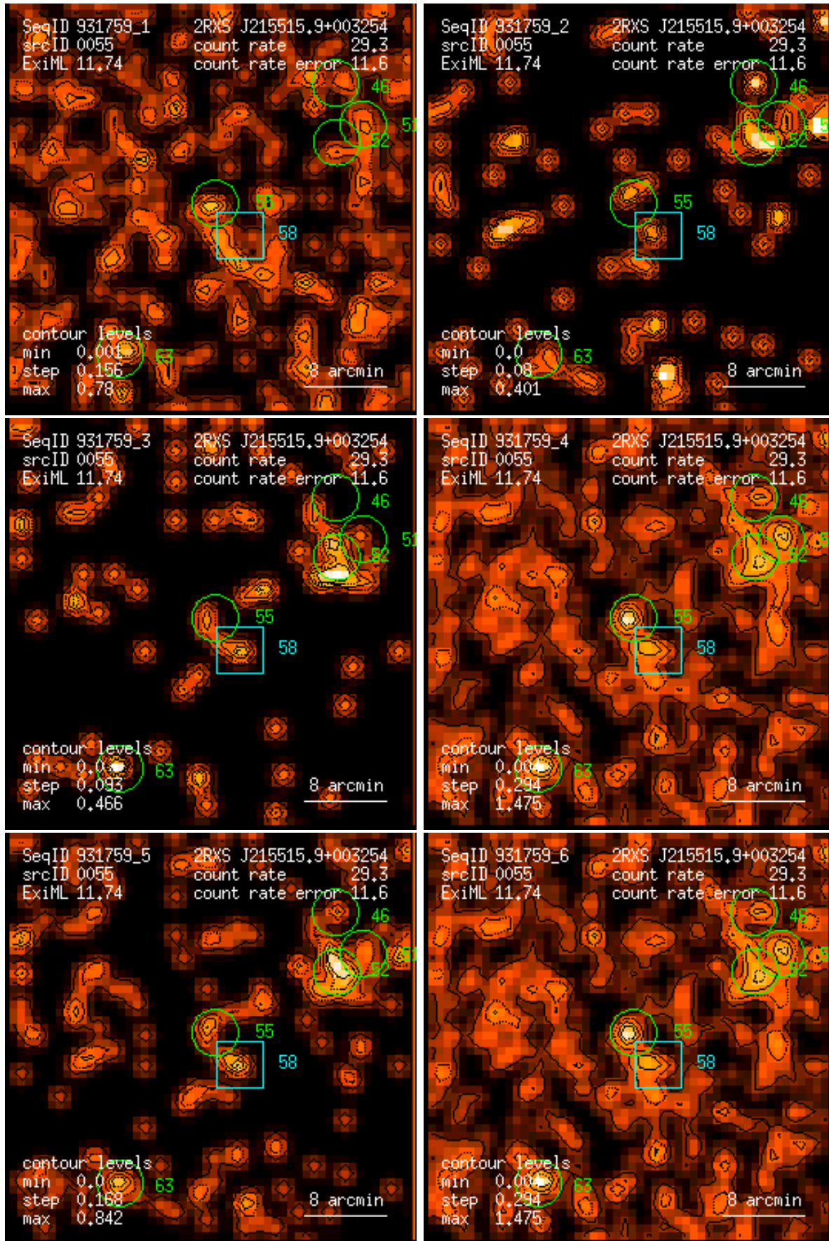
Figure 55: RASS 931759: detection 0055: band rate images, Gaussian filter: (1) PSPC channels 11 – 41, (2) 52 – 90, (3) 91 – 201, (4) 11 – 235, (5) 52 – 201, (6) 11 – 201. Broad band rates in counts/ks. Band rate contour levels in counts/ks/arcmin 2 .
