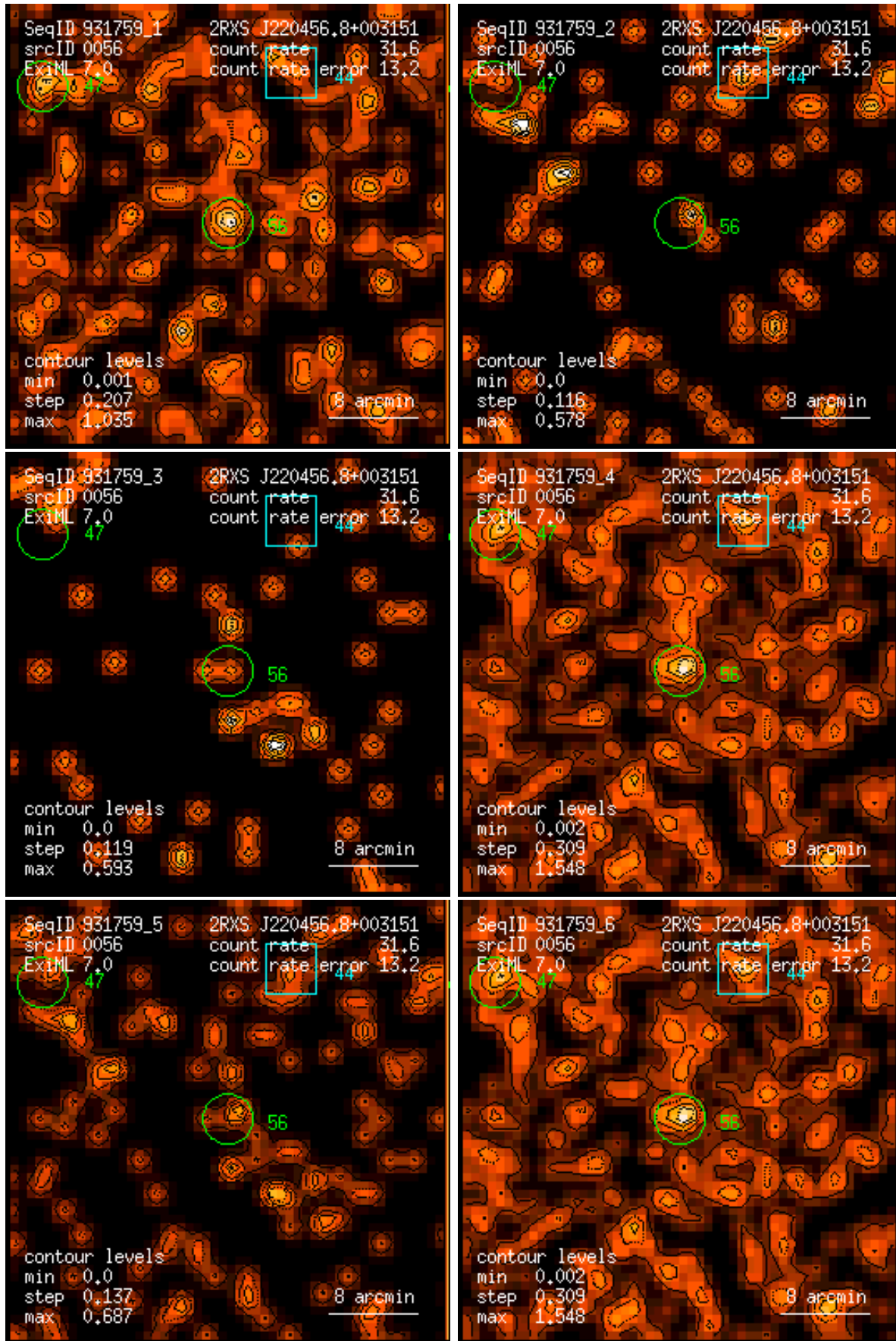
Figure 56: RASS 931759: detection 0056: band rate images, Gaussian filter: (1) PSPC channels 11 – 41, (2) 52 – 90, (3) 91 – 201, (4) 11 – 235, (5) 52 – 201, (6) 11 – 201. Broad band rates in counts/ks. Band rate contour levels in counts/ks/arcmin 2 .
