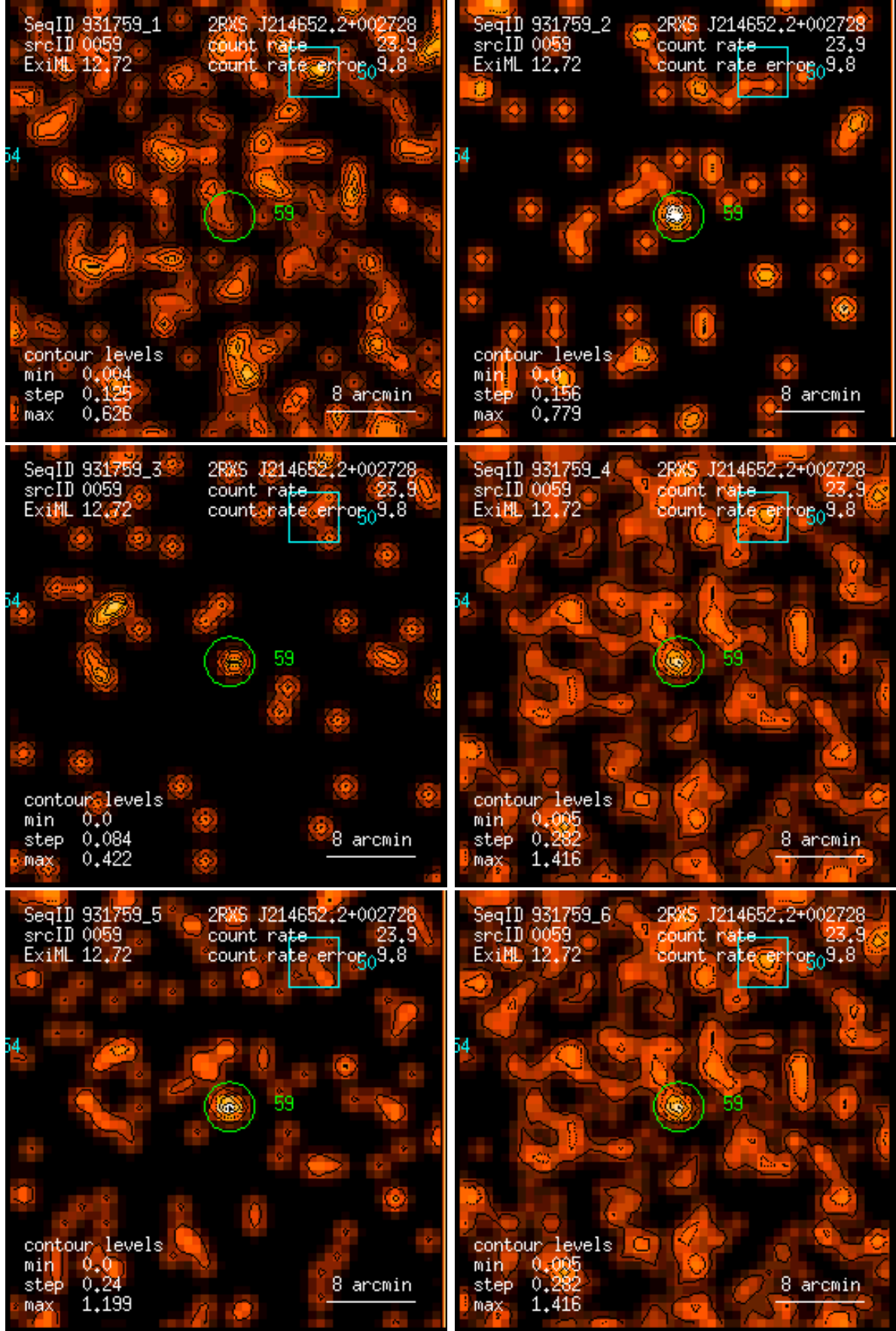
Figure 59: RASS 931759: detection 0059: band rate images, Gaussian filter: (1) PSPC channels 11 – 41, (2) 52 – 90, (3) 91 – 201, (4) 11 – 235, (5) 52 – 201, (6) 11 – 201. Broad band rates in counts/ks. Band rate contour levels in counts/ks/arcmin 2 .
