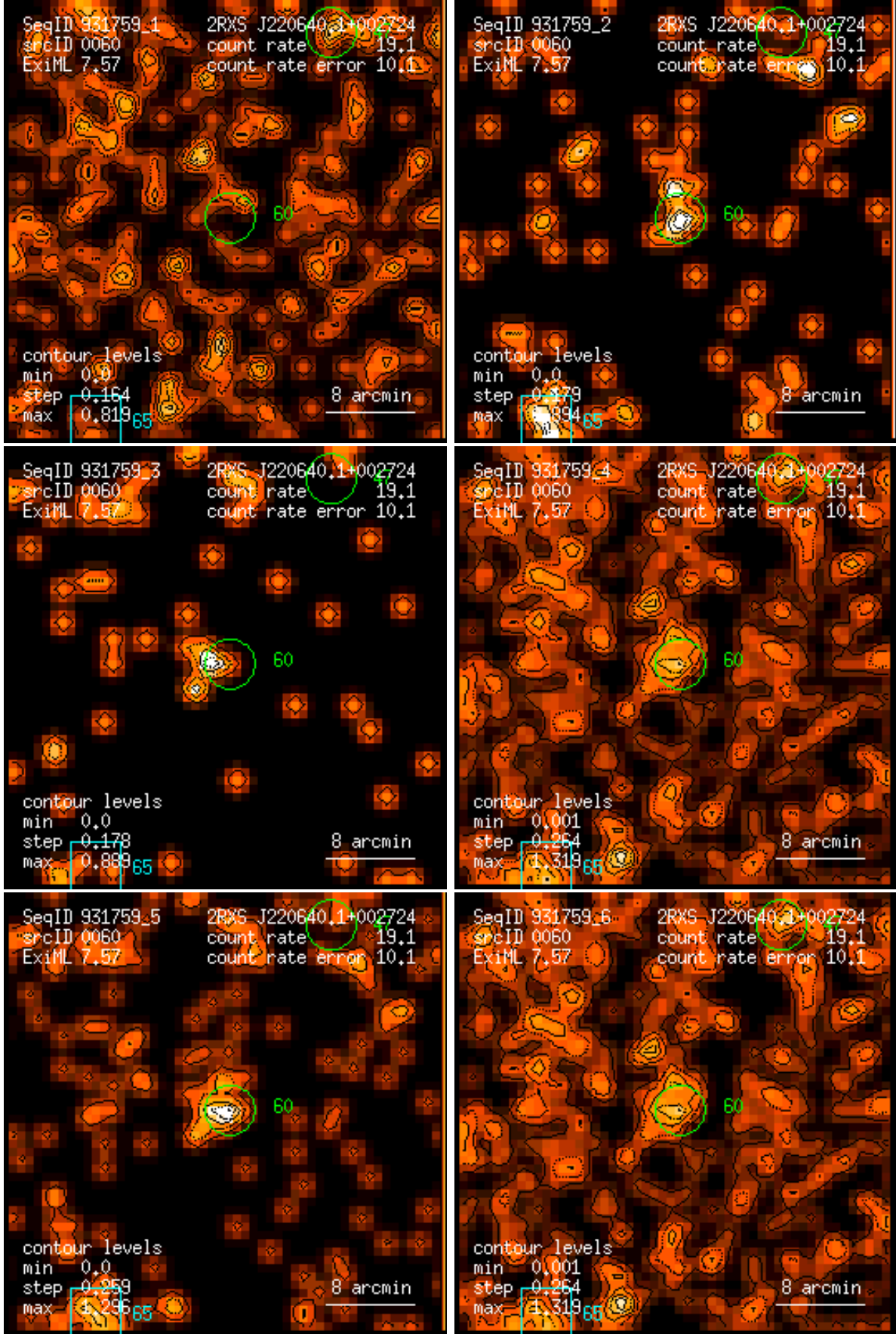
Figure 60: RASS 931759: detection 0060: band rate images, Gaussian filter: (1) PSPC channels 11 – 41, (2) 52 – 90, (3) 91 – 201, (4) 11 – 235, (5) 52 – 201, (6) 11 – 201. Broad band rates in counts/ks. Band rate contour levels in counts/ks/arcmin 2 .
