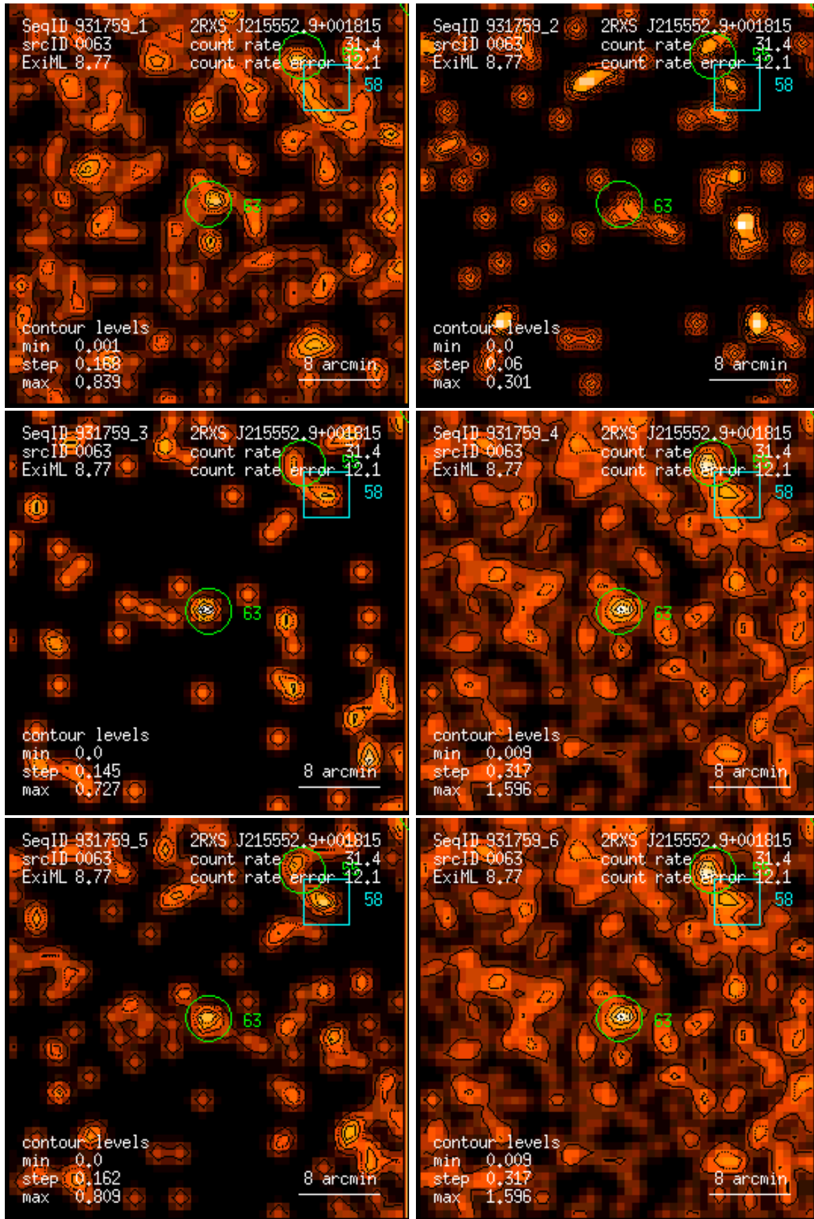
Figure 63: RASS 931759: detection 0063: band rate images, Gaussian filter: (1) PSPC channels 11 – 41, (2) 52 – 90, (3) 91 – 201, (4) 11 – 235, (5) 52 – 201, (6) 11 – 201. Broad band rates in counts/ks. Band rate contour levels in counts/ks/arcmin 2 .
