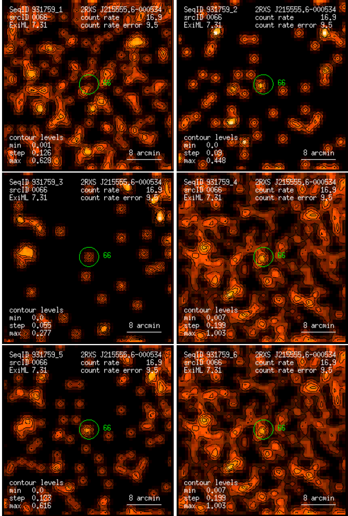
Figure 66: RASS 931759: detection 0066: band rate images, Gaussian filter: (1) PSPC channels 11 – 41, (2) 52 – 90, (3) 91 – 201, (4) 11 – 235, (5) 52 – 201, (6) 11 – 201. Broad band rates in counts/ks. Band rate contour levels in counts/ks/arcmin 2 .
