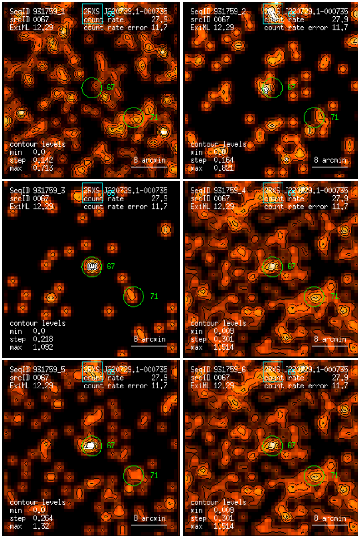
Figure 67: RASS 931759: detection 0067: band rate images, Gaussian filter: (1) PSPC channels 11 – 41, (2) 52 – 90, (3) 91 – 201, (4) 11 – 235, (5) 52 – 201, (6) 11 – 201. Broad band rates in counts/ks. Band rate contour levels in counts/ks/arcmin 2 .
