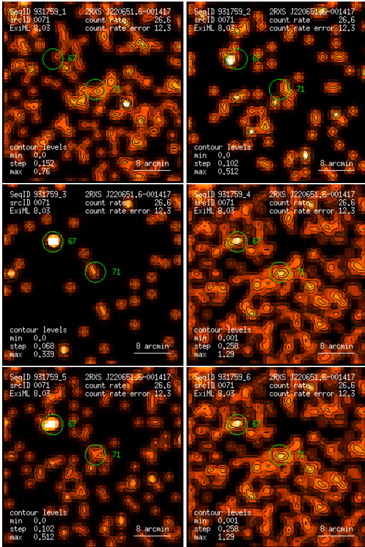
Figure 71: RASS 931759: detection 0071: band rate images, Gaussian filter: (1) PSPC channels 11 – 41, (2) 52 – 90, (3) 91 – 201, (4) 11 – 235, (5) 52 – 201, (6) 11 – 201. Broad band rates in counts/ks. Band rate contour levels in counts/ks/arcmin 2 .
