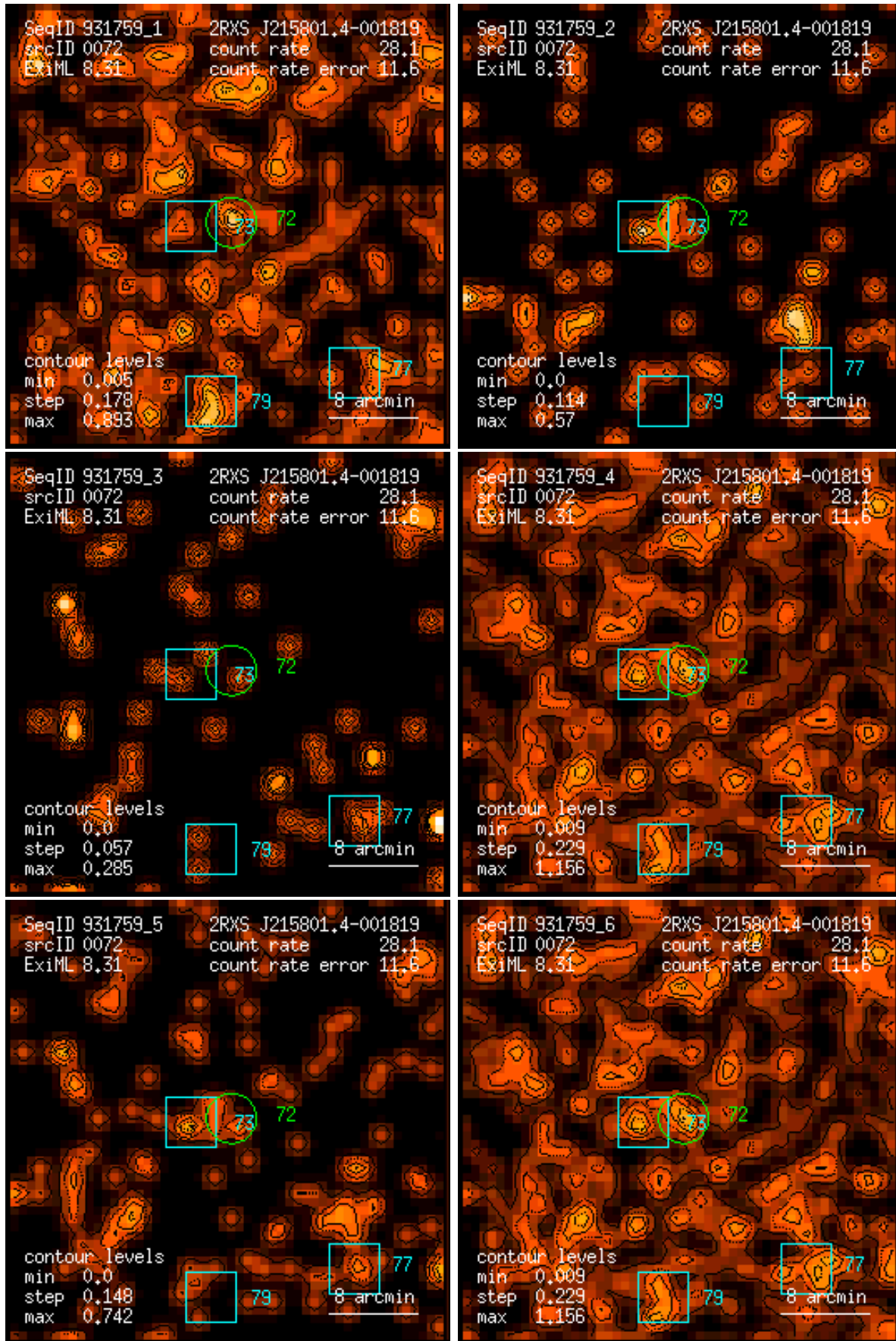
Figure 72: RASS 931759: detection 0072: band rate images, Gaussian filter: (1) PSPC channels 11 – 41, (2) 52 – 90, (3) 91 – 201, (4) 11 – 235, (5) 52 – 201, (6) 11 – 201. Broad band rates in counts/ks. Band rate contour levels in counts/ks/arcmin 2 .
