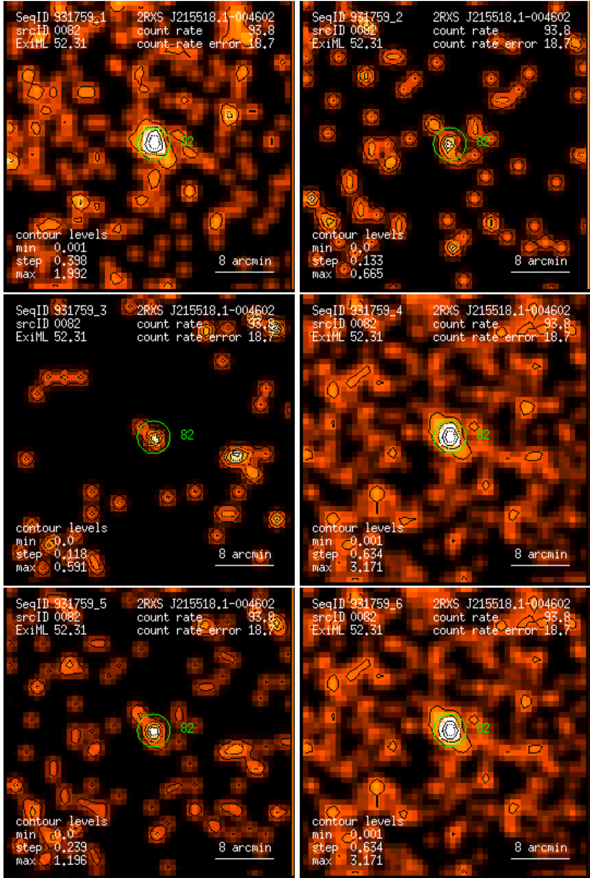
Figure 82: RASS 931759: detection 0082: band rate images, Gaussian filter: (1) PSPC channels 11 – 41, (2) 52 – 90, (3) 91 – 201, (4) 11 – 235, (5) 52 – 201, (6) 11 – 201. Broad band rates in counts/ks. Band rate contour levels in counts/ks/arcmin 2 .
