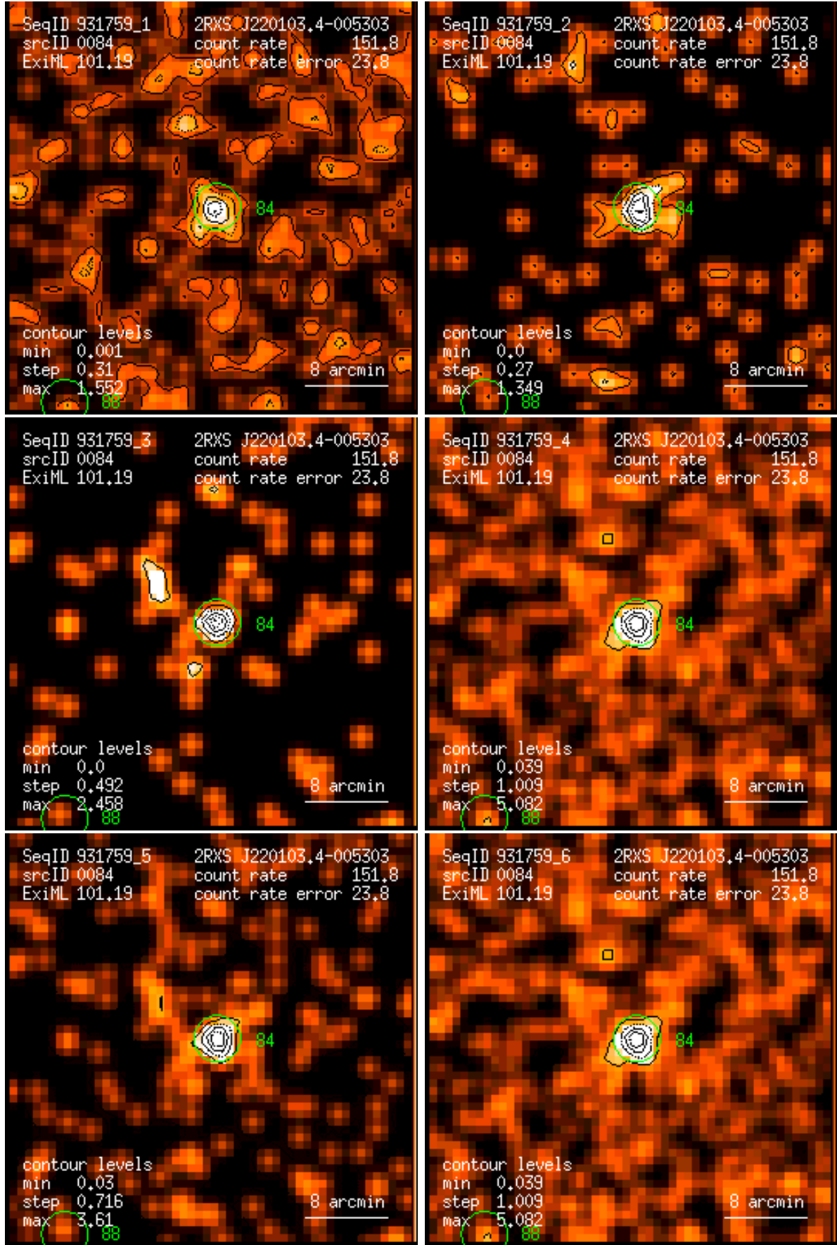
Figure 84: RASS 931759: detection 0084: band rate images, Gaussian filter: (1) PSPC channels 11 – 41, (2) 52 – 90, (3) 91 – 201, (4) 11 – 235, (5) 52 – 201, (6) 11 – 201. Broad band rates in counts/ks. Band rate contour levels in counts/ks/arcmin 2 .
