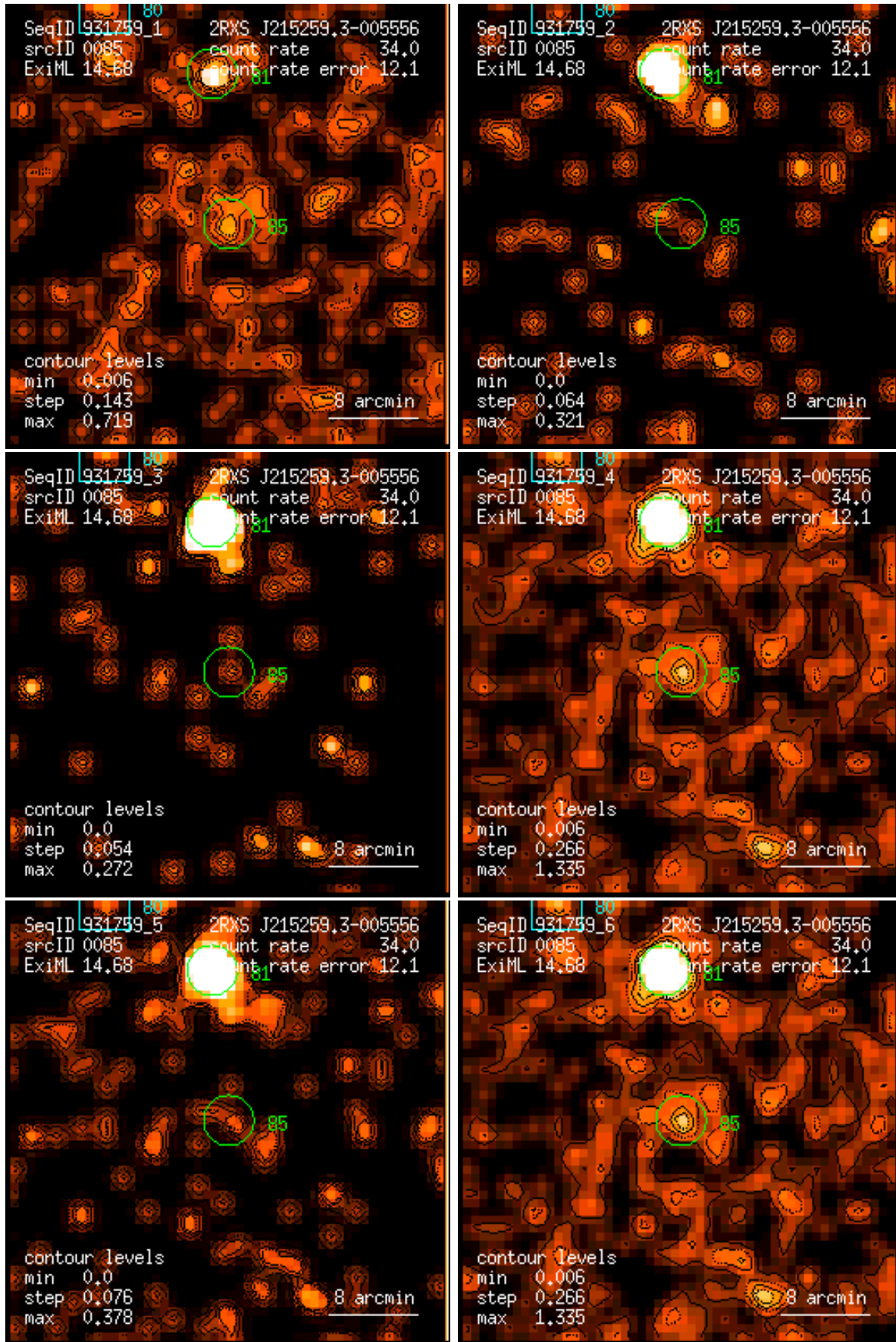
Figure 85: RASS 931759: detection 0085: band rate images, Gaussian filter: (1) PSPC channels 11 – 41, (2) 52 – 90, (3) 91 – 201, (4) 11 – 235, (5) 52 – 201, (6) 11 – 201. Broad band rates in counts/ks. Band rate contour levels in counts/ks/arcmin 2 .
