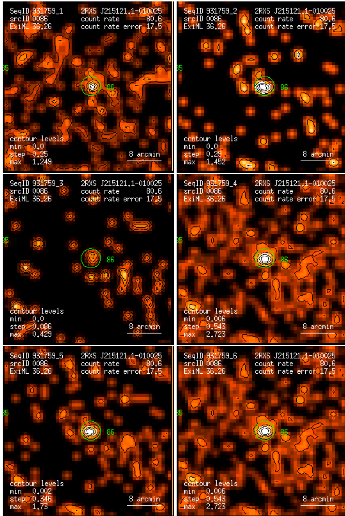
Figure 86: RASS 931759: detection 0086: band rate images, Gaussian filter: (1) PSPC channels 11 – 41, (2) 52 – 90, (3) 91 – 201, (4) 11 – 235, (5) 52 – 201, (6) 11 – 201. Broad band rates in counts/ks. Band rate contour levels in counts/ks/arcmin 2 .
