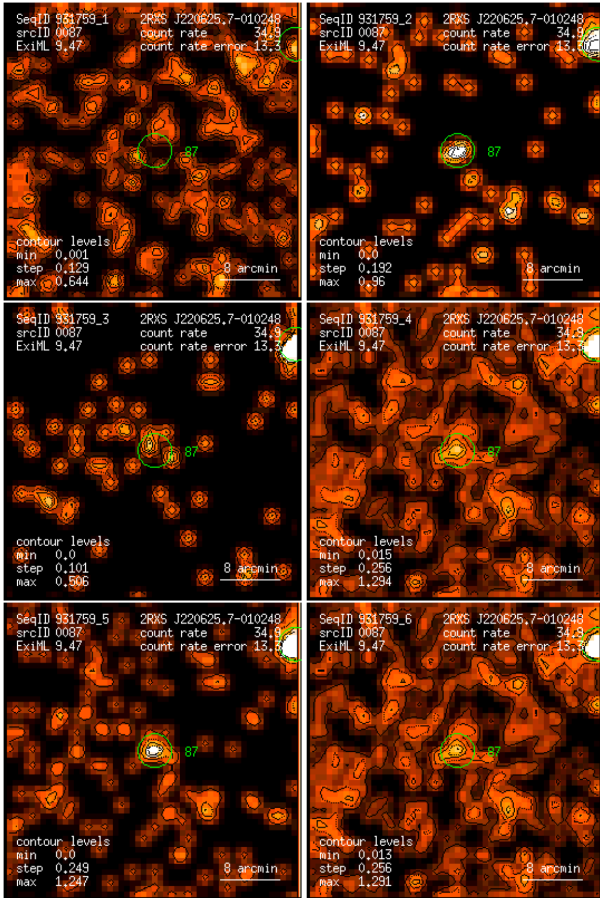
Figure 87: RASS 931759: detection 0087: band rate images, Gaussian filter: (1) PSPC channels 11 – 41, (2) 52 – 90, (3) 91 – 201, (4) 11 – 235, (5) 52 – 201, (6) 11 – 201. Broad band rates in counts/ks. Band rate contour levels in counts/ks/arcmin 2 .
