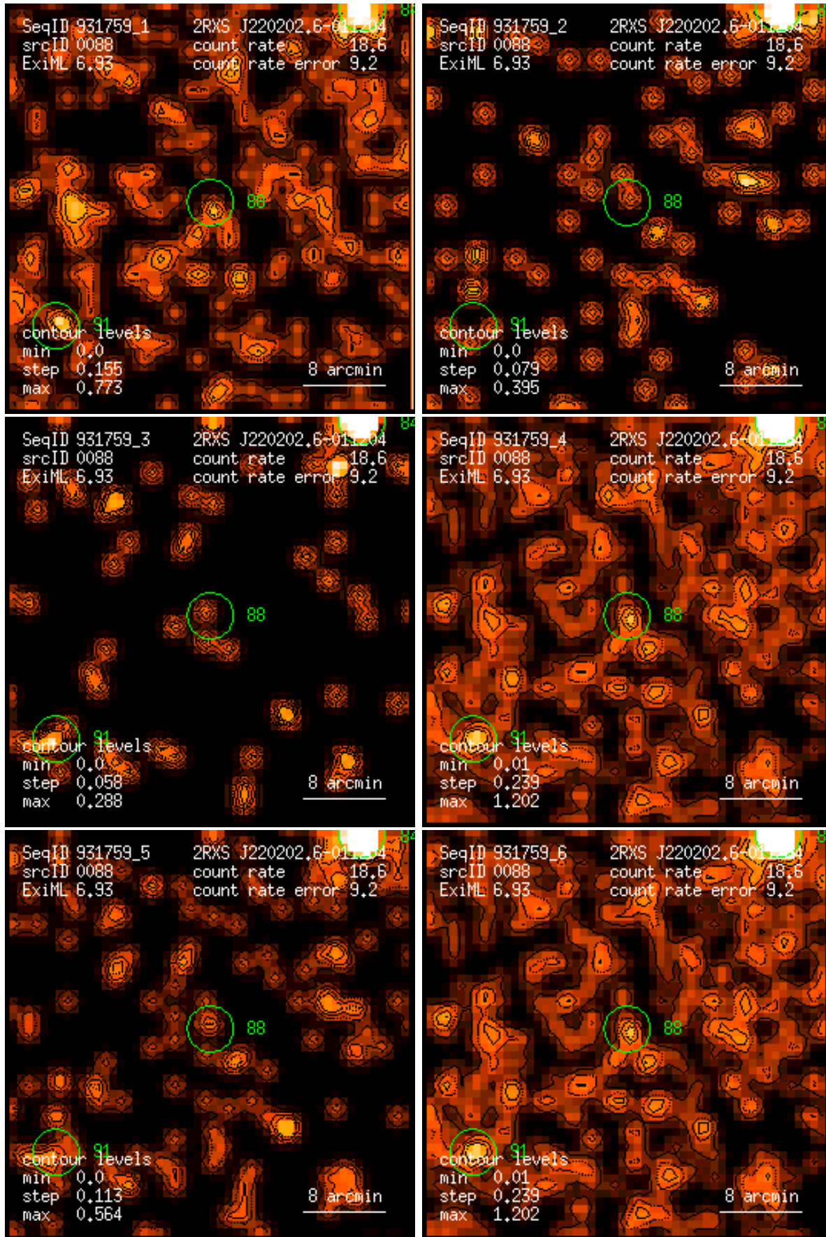
Figure 88: RASS 931759: detection 0088: band rate images, Gaussian filter: (1) PSPC channels 11 – 41, (2) 52 – 90, (3) 91 – 201, (4) 11 – 235, (5) 52 – 201, (6) 11 – 201. Broad band rates in counts/ks. Band rate contour levels in counts/ks/arcmin 2 .
