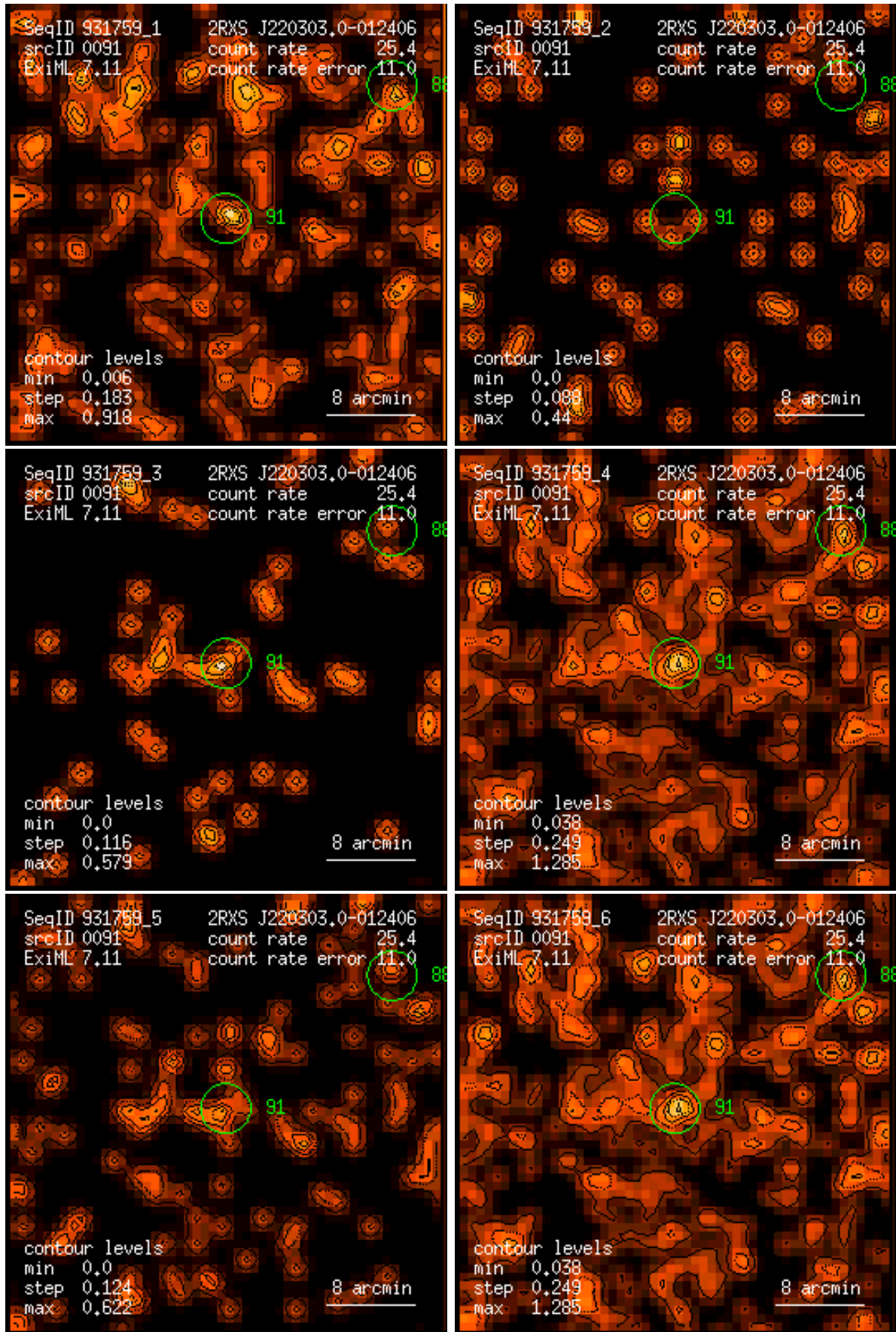
Figure 91: RASS 931759: detection 0091: band rate images, Gaussian filter: (1) PSPC channels 11 – 41, (2) 52 – 90, (3) 91 – 201, (4) 11 – 235, (5) 52 – 201, (6) 11 – 201. Broad band rates in counts/ks. Band rate contour levels in counts/ks/arcmin 2 .
