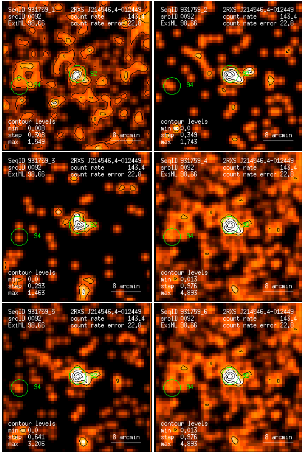
Figure 92: RASS 931759: detection 0092: band rate images, Gaussian filter: (1) PSPC channels 11 – 41, (2) 52 – 90, (3) 91 – 201, (4) 11 – 235, (5) 52 – 201, (6) 11 – 201. Broad band rates in counts/ks. Band rate contour levels in counts/ks/arcmin 2 .
