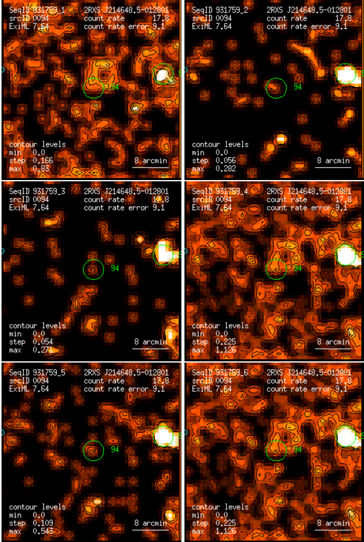
Figure 94: RASS 931759: detection 0094: band rate images, Gaussian filter: (1) PSPC channels 11 – 41, (2) 52 – 90, (3) 91 – 201, (4) 11 – 235, (5) 52 – 201, (6) 11 – 201. Broad band rates in counts/ks. Band rate contour levels in counts/ks/arcmin 2 .
