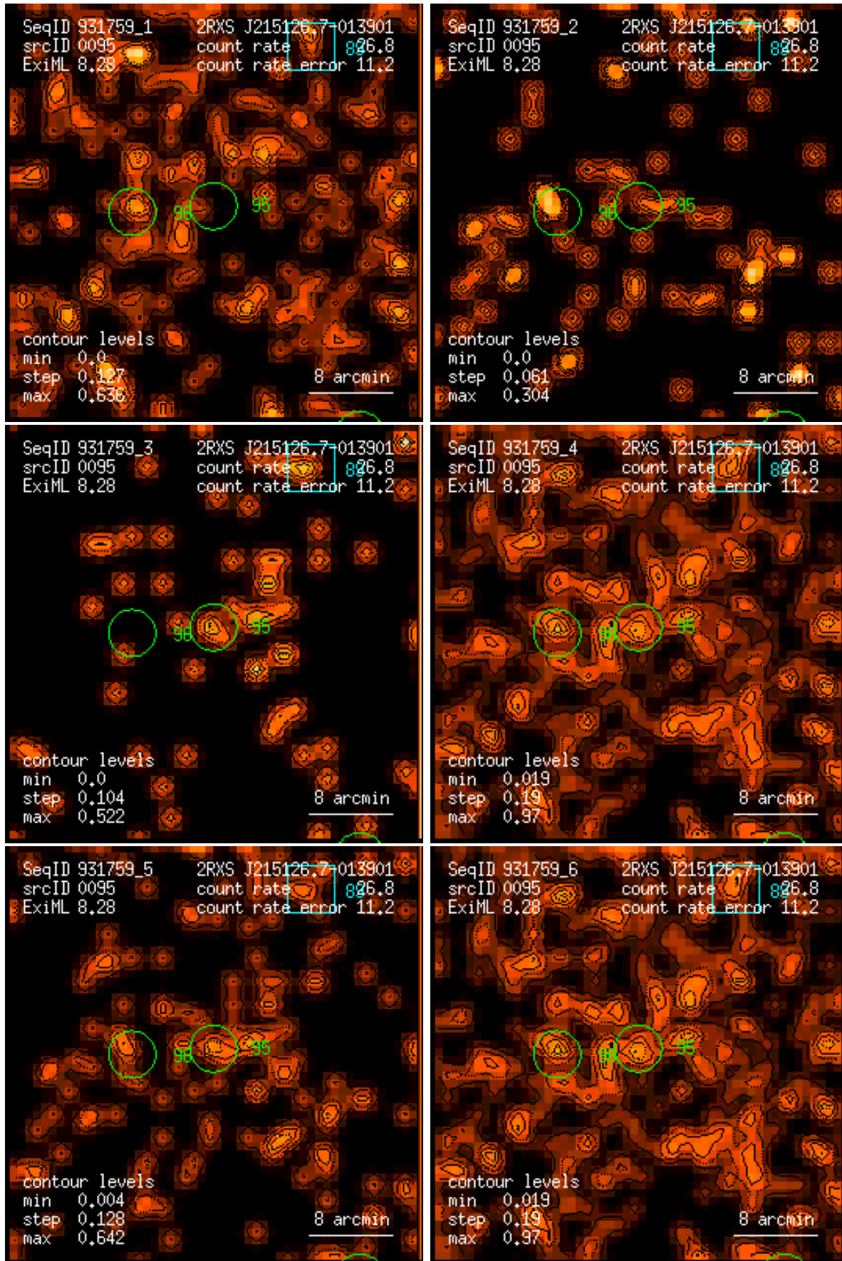
Figure 95: RASS 931759: detection 0095: band rate images, Gaussian filter: (1) PSPC channels 11 – 41, (2) 52 – 90, (3) 91 – 201, (4) 11 – 235, (5) 52 – 201, (6) 11 – 201. Broad band rates in counts/ks. Band rate contour levels in counts/ks/arcmin 2 .
