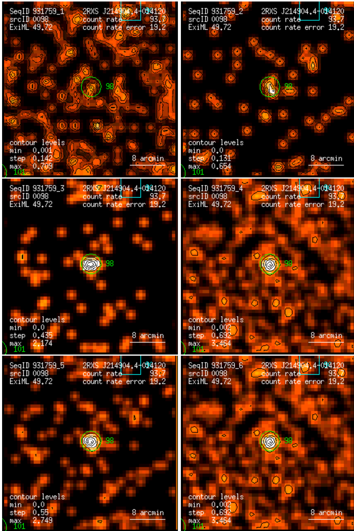
Figure 98: RASS 931759: detection 0098: band rate images, Gaussian filter: (1) PSPC channels 11 – 41, (2) 52 – 90, (3) 91 – 201, (4) 11 – 235, (5) 52 – 201, (6) 11 – 201. Broad band rates in counts/ks. Band rate contour levels in counts/ks/arcmin 2 .
