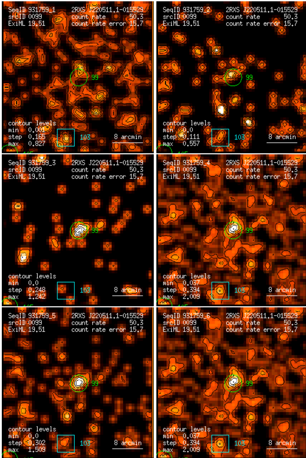
Figure 99: RASS 931759: detection 0099: band rate images, Gaussian filter: (1) PSPC channels 11 – 41, (2) 52 – 90, (3) 91 – 201, (4) 11 – 235, (5) 52 – 201, (6) 11 – 201. Broad band rates in counts/ks. Band rate contour levels in counts/ks/arcmin 2 .
