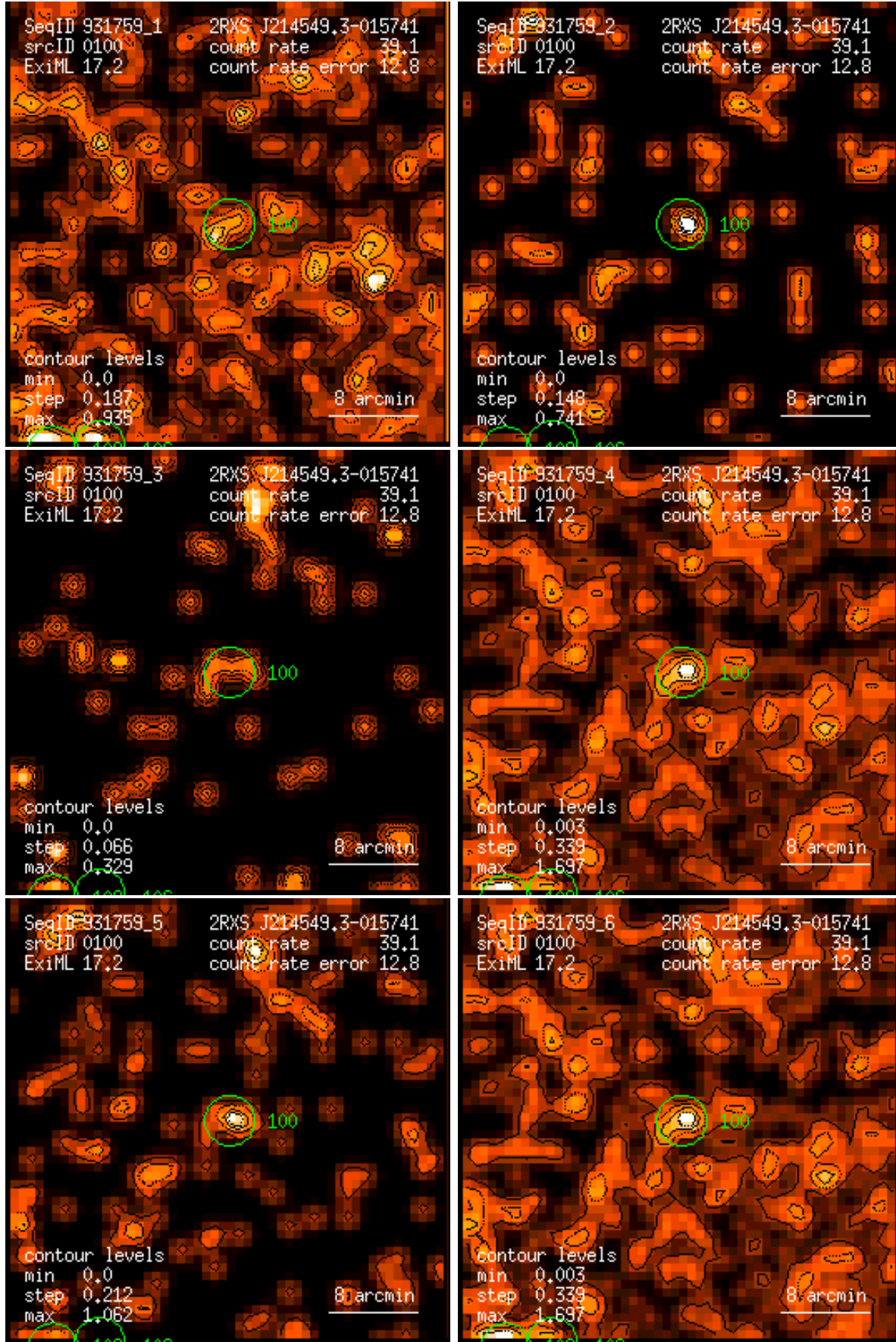
Figure 100: RASS 931759: detection 0100: band rate images, Gaussian filter: (1) PSPC channels 11 – 41, (2) 52 – 90, (3) 91 – 201, (4) 11 – 235, (5) 52 – 201, (6) 11 – 201. Broad band rates in counts/ks. Band rate contour levels in counts/ks/arcmin 2 .
