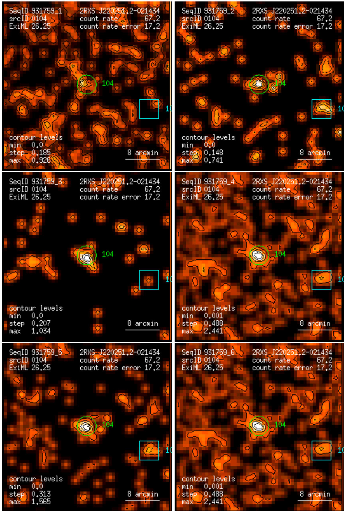
Figure 104: RASS 931759: detection 0104: band rate images, Gaussian filter: (1) PSPC channels 11 – 41, (2) 52 – 90, (3) 91 – 201, (4) 11 – 235, (5) 52 – 201, (6) 11 – 201. Broad band rates in counts/ks. Band rate contour levels in counts/ks/arcmin 2 .
