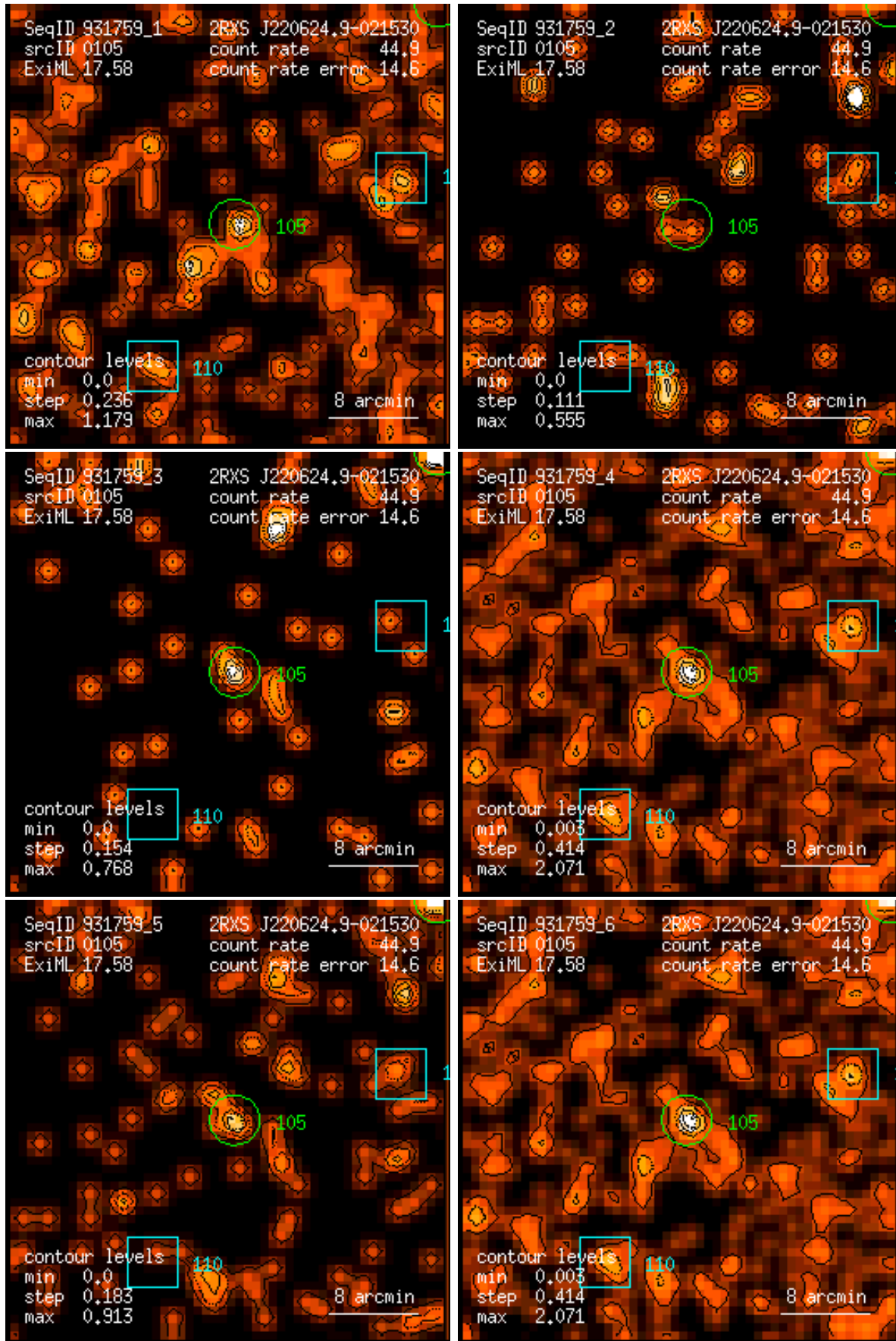
Figure 105: RASS 931759: detection 0105: band rate images, Gaussian filter: (1) PSPC channels 11 – 41, (2) 52 – 90, (3) 91 – 201, (4) 11 – 235, (5) 52 – 201, (6) 11 – 201. Broad band rates in counts/ks. Band rate contour levels in counts/ks/arcmin 2 .
