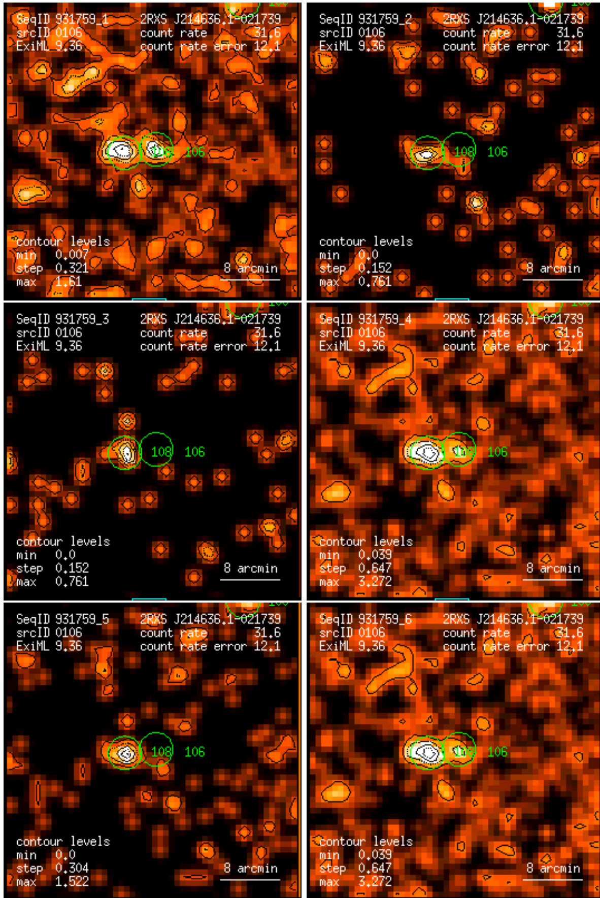
Figure 106: RASS 931759: detection 0106: band rate images, Gaussian filter: (1) PSPC channels 11 – 41, (2) 52 – 90, (3) 91 – 201, (4) 11 – 235, (5) 52 – 201, (6) 11 – 201. Broad band rates in counts/ks. Band rate contour levels in counts/ks/arcmin 2 .
