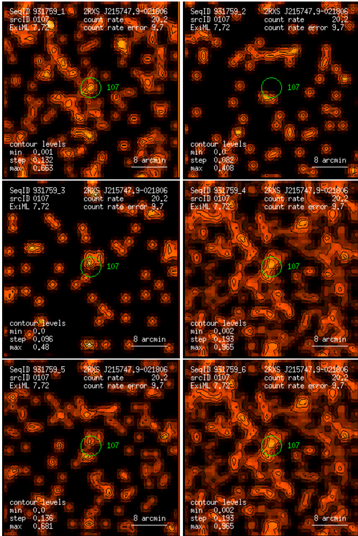
Figure 107: RASS 931759: detection 0107: band rate images, Gaussian filter: (1) PSPC channels 11 – 41, (2) 52 – 90, (3) 91 – 201, (4) 11 – 235, (5) 52 – 201, (6) 11 – 201. Broad band rates in counts/ks. Band rate contour levels in counts/ks/arcmin 2 .
