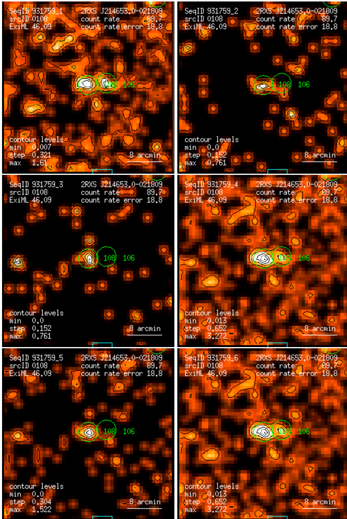
Figure 108: RASS 931759: detection 0108: band rate images, Gaussian filter: (1) PSPC channels 11 – 41, (2) 52 – 90, (3) 91 – 201, (4) 11 – 235, (5) 52 – 201, (6) 11 – 201. Broad band rates in counts/ks. Band rate contour levels in counts/ks/arcmin 2 .
