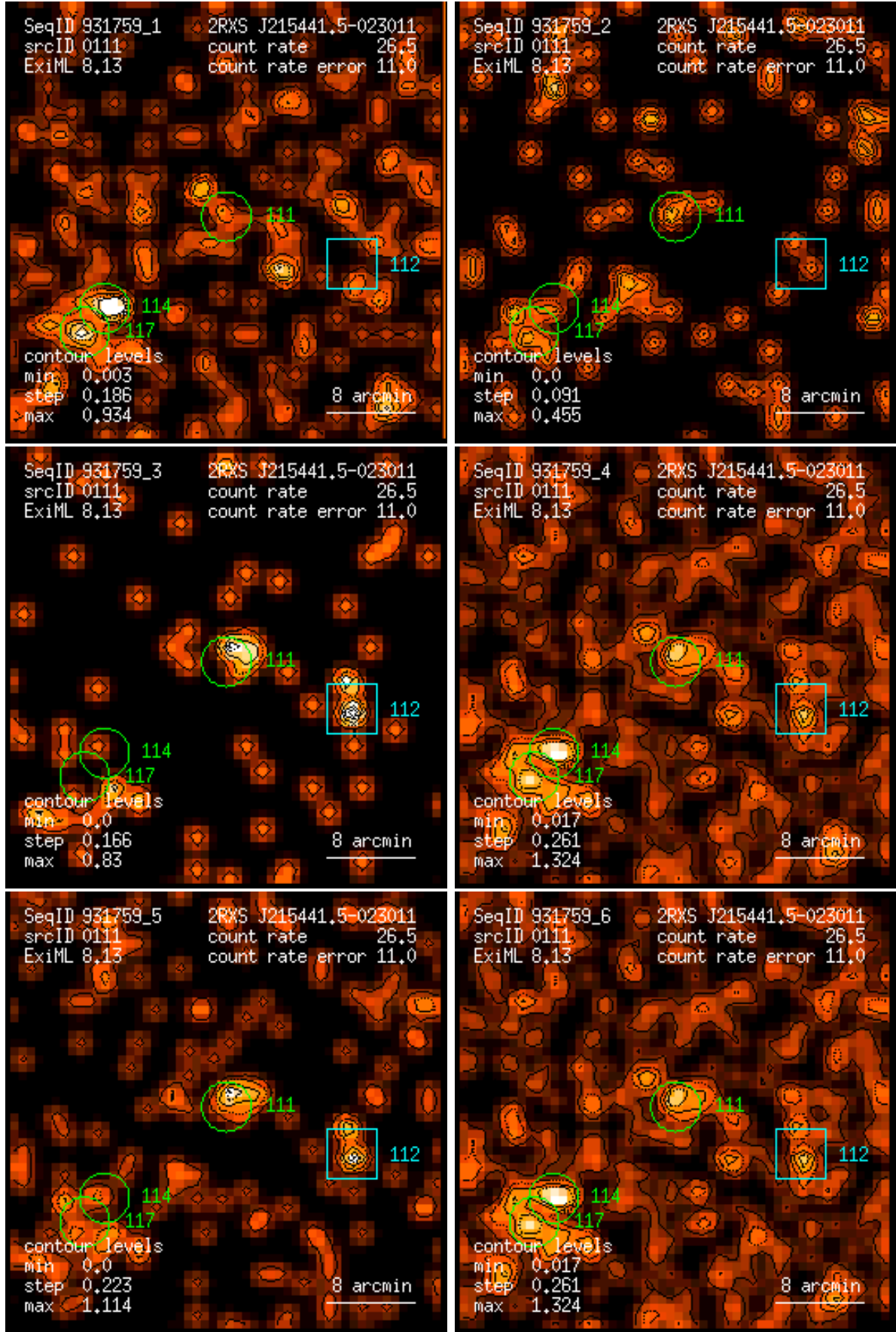
Figure 111: RASS 931759: detection 0111: band rate images, Gaussian filter: (1) PSPC channels 11 – 41, (2) 52 – 90, (3) 91 – 201, (4) 11 – 235, (5) 52 – 201, (6) 11 – 201. Broad band rates in counts/ks. Band rate contour levels in counts/ks/arcmin 2 .
