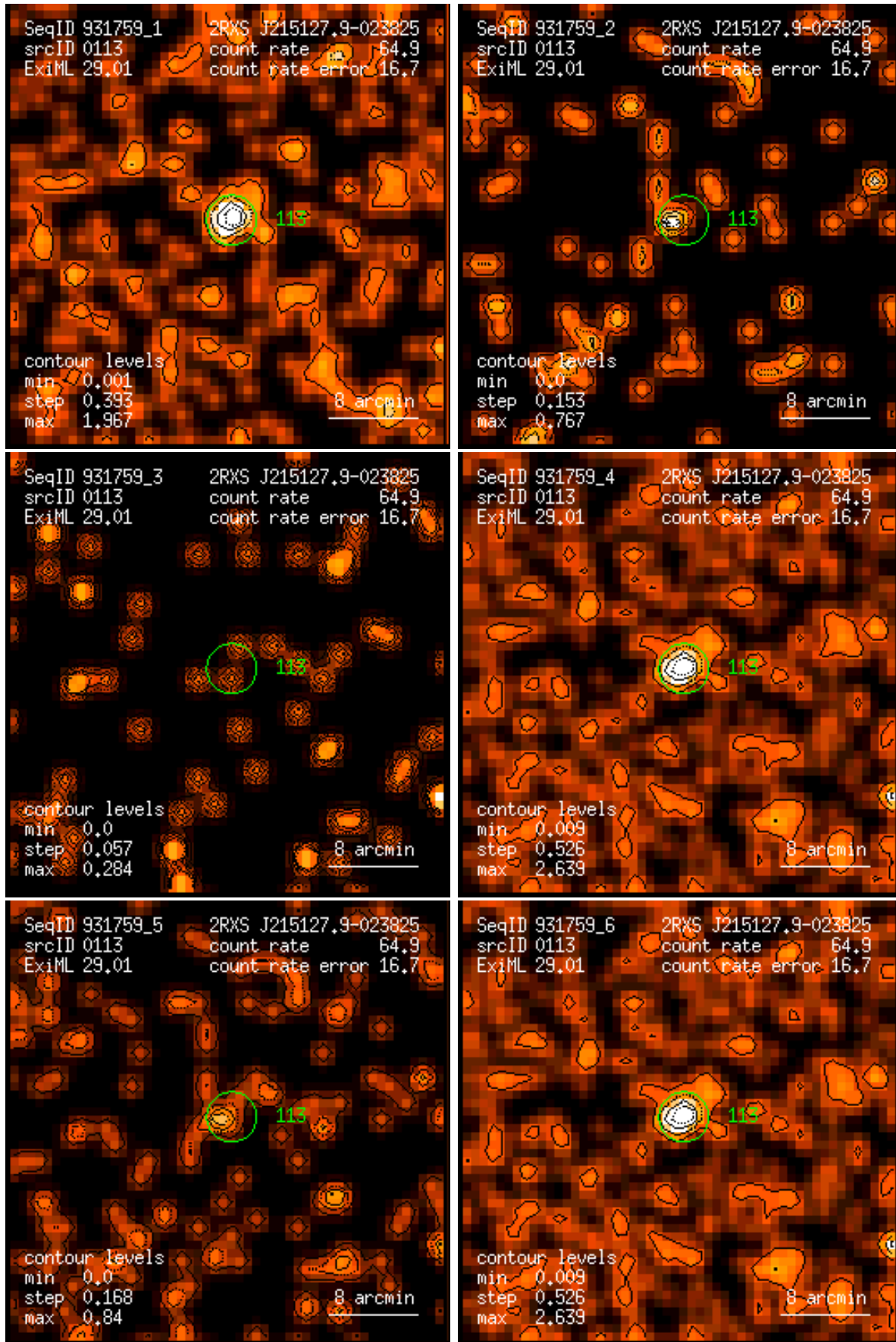
Figure 113: RASS 931759: detection 0113: band rate images, Gaussian filter: (1) PSPC channels 11 – 41, (2) 52 – 90, (3) 91 – 201, (4) 11 – 235, (5) 52 – 201, (6) 11 – 201. Broad band rates in counts/ks. Band rate contour levels in counts/ks/arcmin 2 .
