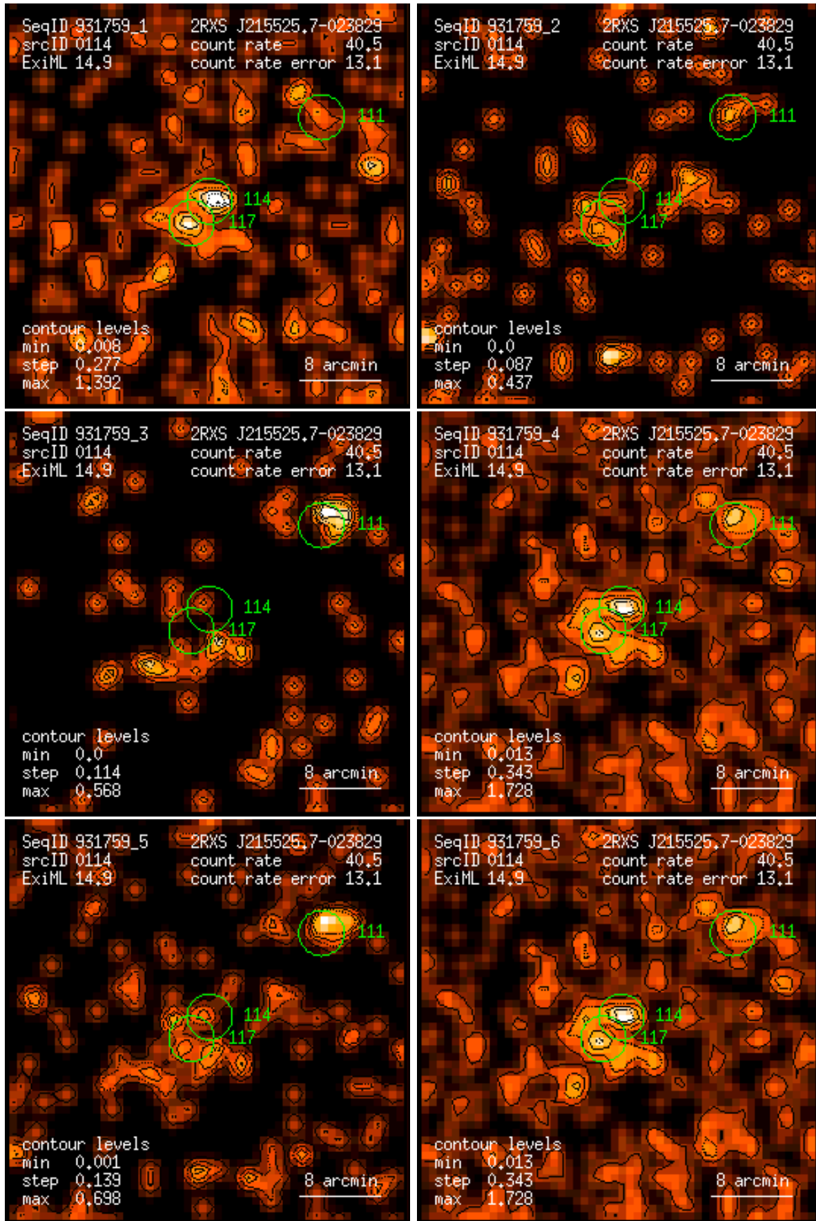
Figure 114: RASS 931759: detection 0114: band rate images, Gaussian filter: (1) PSPC channels 11 – 41, (2) 52 – 90, (3) 91 – 201, (4) 11 – 235, (5) 52 – 201, (6) 11 – 201. Broad band rates in counts/ks. Band rate contour levels in counts/ks/arcmin 2 .
