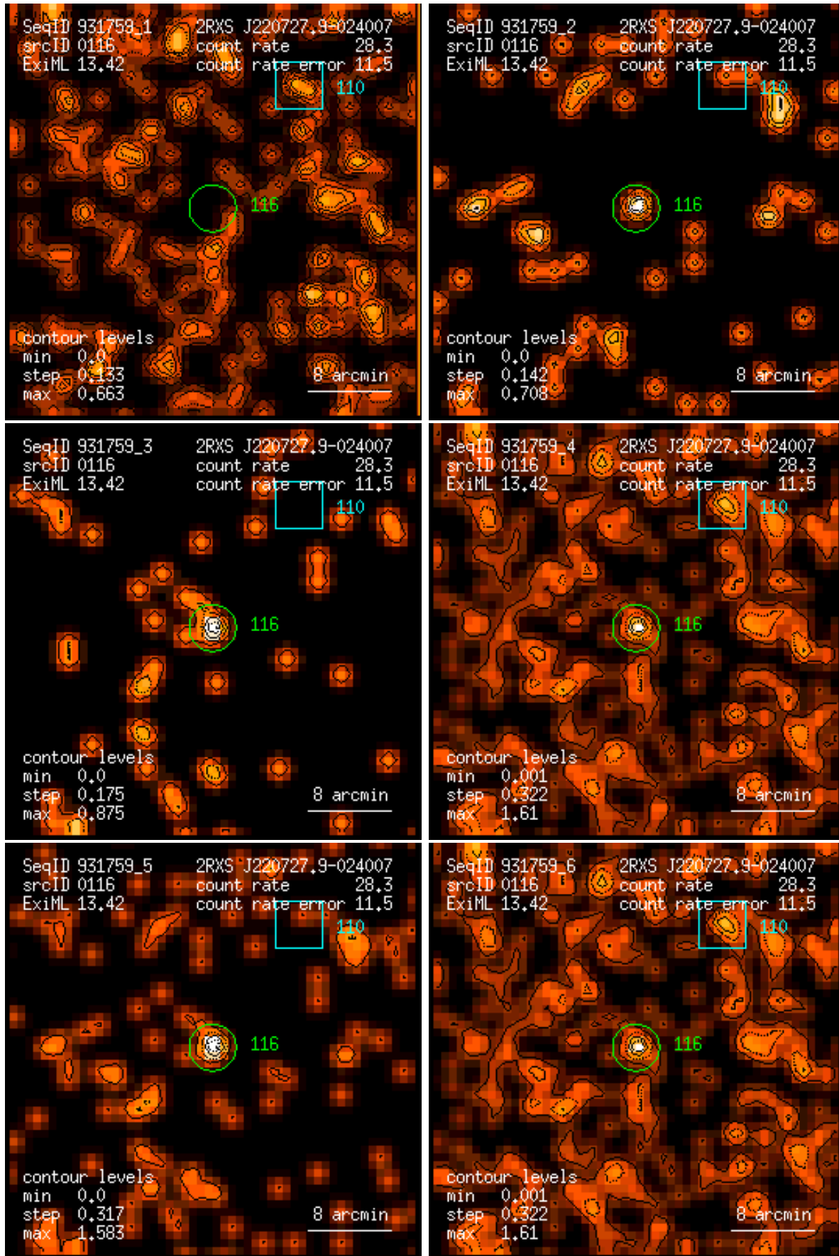
Figure 116: RASS 931759: detection 0116: band rate images, Gaussian filter: (1) PSPC channels 11 – 41, (2) 52 – 90, (3) 91 – 201, (4) 11 – 235, (5) 52 – 201, (6) 11 – 201. Broad band rates in counts/ks. Band rate contour levels in counts/ks/arcmin 2 .
