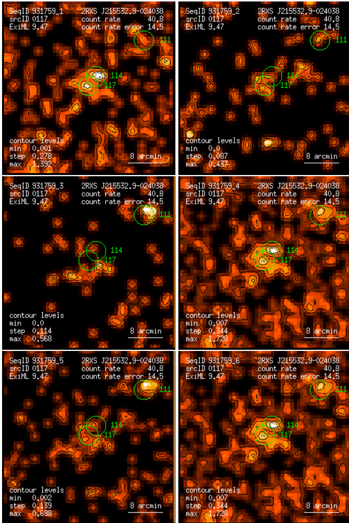
Figure 117: RASS 931759: detection 0117: band rate images, Gaussian filter: (1) PSPC channels 11 – 41, (2) 52 – 90, (3) 91 – 201, (4) 11 – 235, (5) 52 – 201, (6) 11 – 201. Broad band rates in counts/ks. Band rate contour levels in counts/ks/arcmin 2 .
