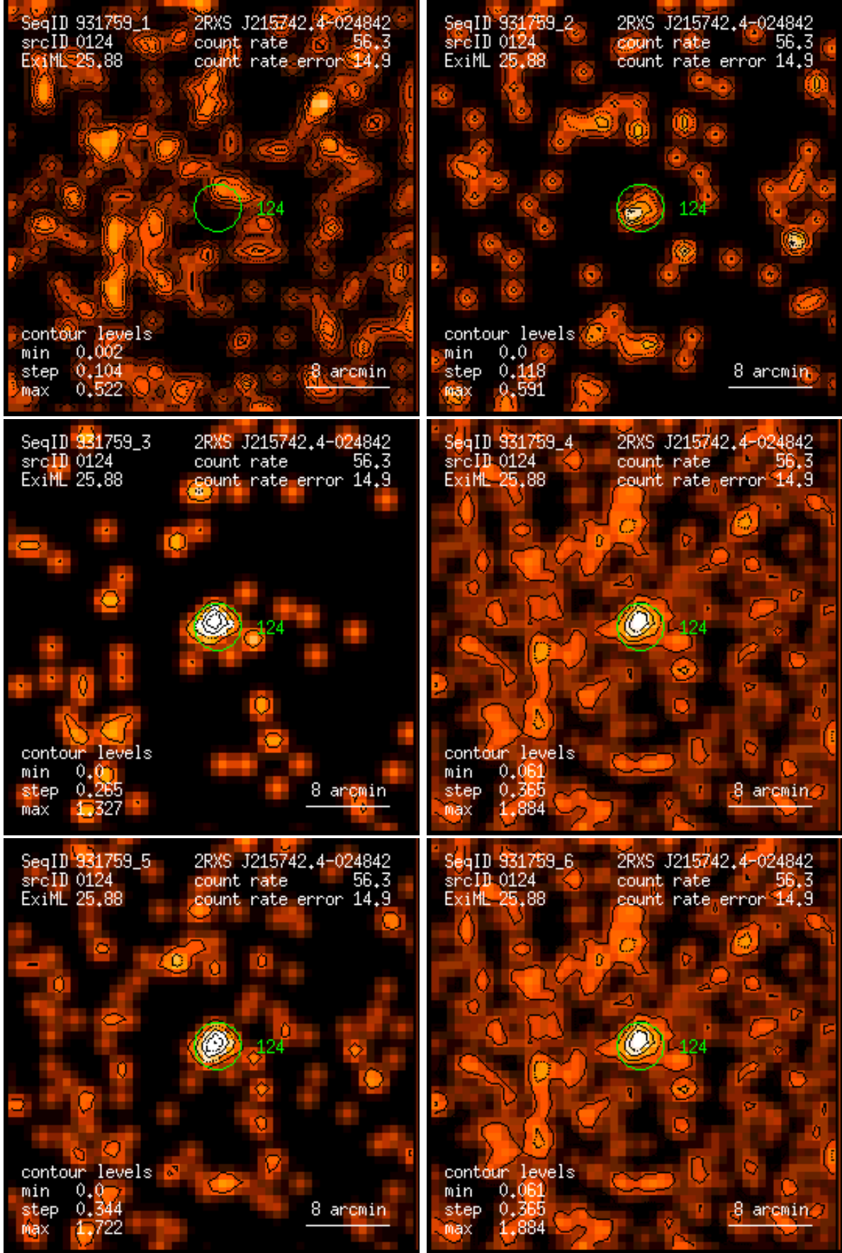
Figure 124: RASS 931759: detection 0124: band rate images, Gaussian filter: (1) PSPC channels 11 – 41, (2) 52 – 90, (3) 91 – 201, (4) 11 – 235, (5) 52 – 201, (6) 11 – 201. Broad band rates in counts/ks. Band rate contour levels in counts/ks/arcmin 2 .
