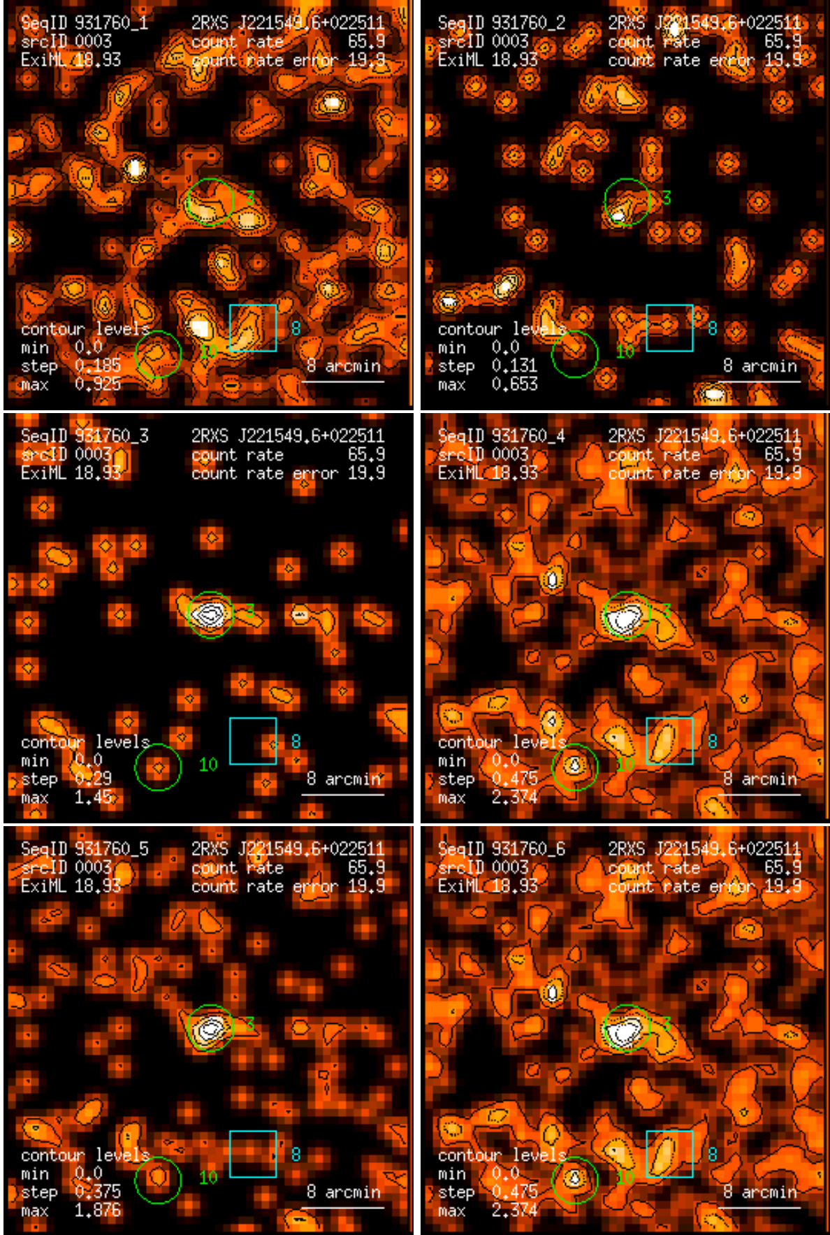
Figure 3: RASS 931760: detection 0003: band rate images, Gaussian filter: (1) PSPC channels 11 – 41, (2) 52 – 90, (3) 91 – 201, (4) 11 – 235, (5) 52 – 201, (6) 11 – 201. Broad band rates in counts/ks. Band rate contour levels in counts/ks/arcmin 2 .
