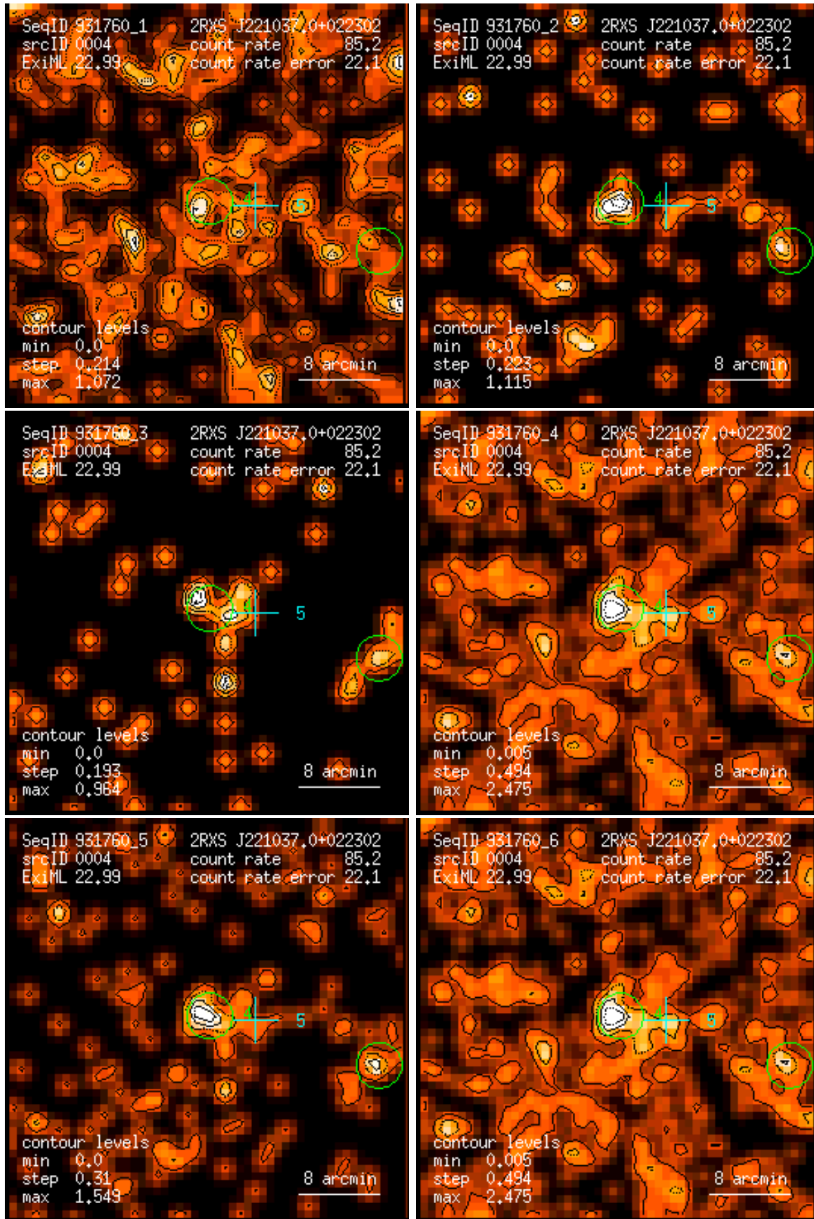
Figure 4: RASS 931760: detection 0004: band rate images, Gaussian filter: (1) PSPC channels 11 – 41, (2) 52 – 90, (3) 91 – 201, (4) 11 – 235, (5) 52 – 201, (6) 11 – 201. Broad band rates in counts/ks. Band rate contour levels in counts/ks/arcmin 2 .
