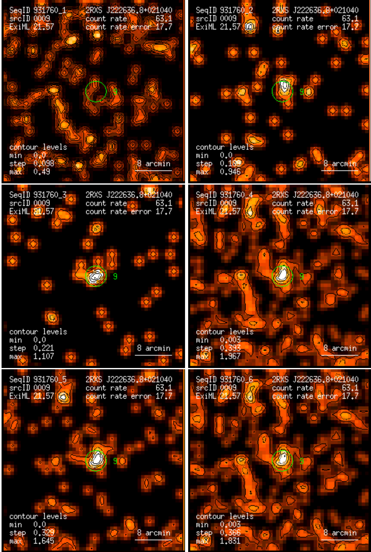
Figure 9: RASS 931760: detection 0009: band rate images, Gaussian filter: (1) PSPC channels 11 – 41, (2) 52 – 90, (3) 91 – 201, (4) 11 – 235, (5) 52 – 201, (6) 11 – 201. Broad band rates in counts/ks. Band rate contour levels in counts/ks/arcmin 2 .
